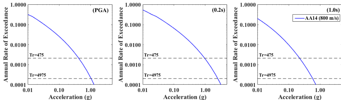
Figure 3. Target hazard curve on rock ( V_s=800 m/s) at the Euroseistest calculated using the Akkar et al., 2014 GMPE (AA14) for three different spectral periods (PGA, 0.2s, 1.0s).
