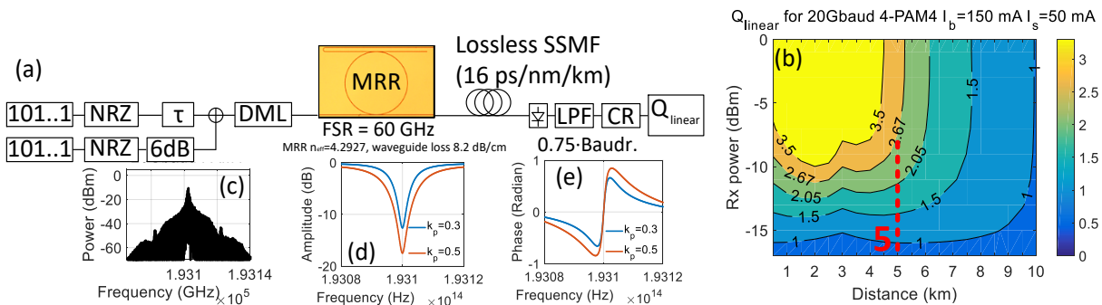
Fig. 1. (a) System under investigation; (b) Q_{\text{linear}} as a function of received power and transmission distance for 20 Gbaud 4-PAM with directly modulated laser; (c) spectrum for 20 Gbaud 4-PAM; MRR transfer function: (d) amplitude and (e) phase.
