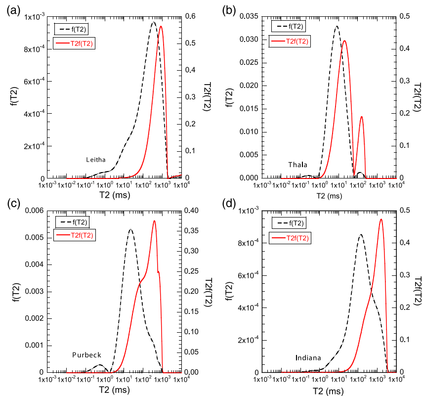
Figure 4. T_2 relaxation time distribution, f(T_2) (dashed black line), and the T_2 -weighted probability distribution function, T_2f(T_2) (solid red line), inferred from NMR measurements on undeformed samples of (a) Leitha, (b) Thala, (c) Purbeck, and (d) Indiana limestones.
