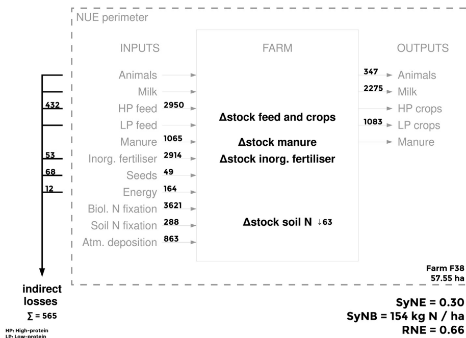
Fig. 3. Example of a diagram produced by the SyNE calculator, showing net nitrogen (N) inputs, net indirect N losses, net N outputs, change in soil N, and the three N-related indicators (System N Efficiency, SyNE; System N Balance, SyNB; Relative N Efficiency, RNE) computed by the calculator. All values are expressed in kg N, except for SyNE and RNE, which are unitless, and for SyNB, which is expressed in kg N ha -1 . Net inputs, net indirect losses, and net outputs are explained in Godinot et al. (2014).
