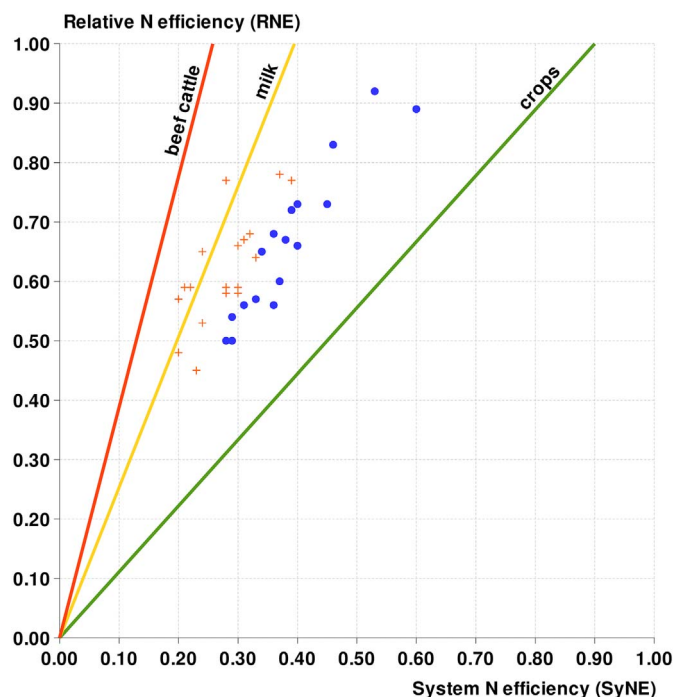
Fig. 2. Comparison between Relative Nitrogen Efficiency (RNE) (unitless) and System Nitrogen Efficiency (SyNE) (unitless) for 38 mixed crop and dairy farms in Brittany. Farm data come from Godinot et al. (2014) and are available in Carof and Godinot (submitted). Diagonal lines represent relationships between RNE and SyNE for specialized farming systems with 100% RNE, equal to potential efficiency for a given product (Godinot et al., 2015). Orange crosses represent farming systems producing > 50% of their nitrogen (N) outputs as animal products, while blue circles represent those producing > 50% of their N outputs as crops. Three outliers with RNE > 1 are not shown.
