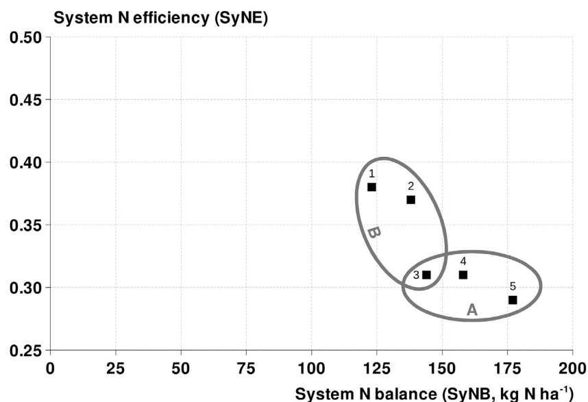
Fig. 4. Relationship between System Nitrogen Efficiency (SyNE) (unitless) and System Nitrogen Balance (SyNB) (kg nitrogen (N) \text{ha}^{-1} ) for 5 mixed dairy-crop farms in a fictive farm support group. A farm advisor could identify sub-group A, whose strategy is to decrease SyNB without decreasing SyNE. For instance, farms 4 and 5 could adopt some management practices of farm 3 (e.g., decrease fertilizer use, decrease change in soil N). Another sub-group (B) could be identified whose strategy is to increase SyNE without decreasing SyNB. For instance, farm 3 could adopt some management practices of farms 1 and 2 (e.g., increase crop production while using fewer fertilizers and more legumes to fix N). Net N inputs, net indirect N losses, net N outputs, change in soil N, SyNE, and SyNB are computed by the calculator using data described by Godinot et al. (2014) and available in Carof and Godinot (submitted). Net inputs, net indirect losses, and net outputs are explained in Godinot et al. (2014).
