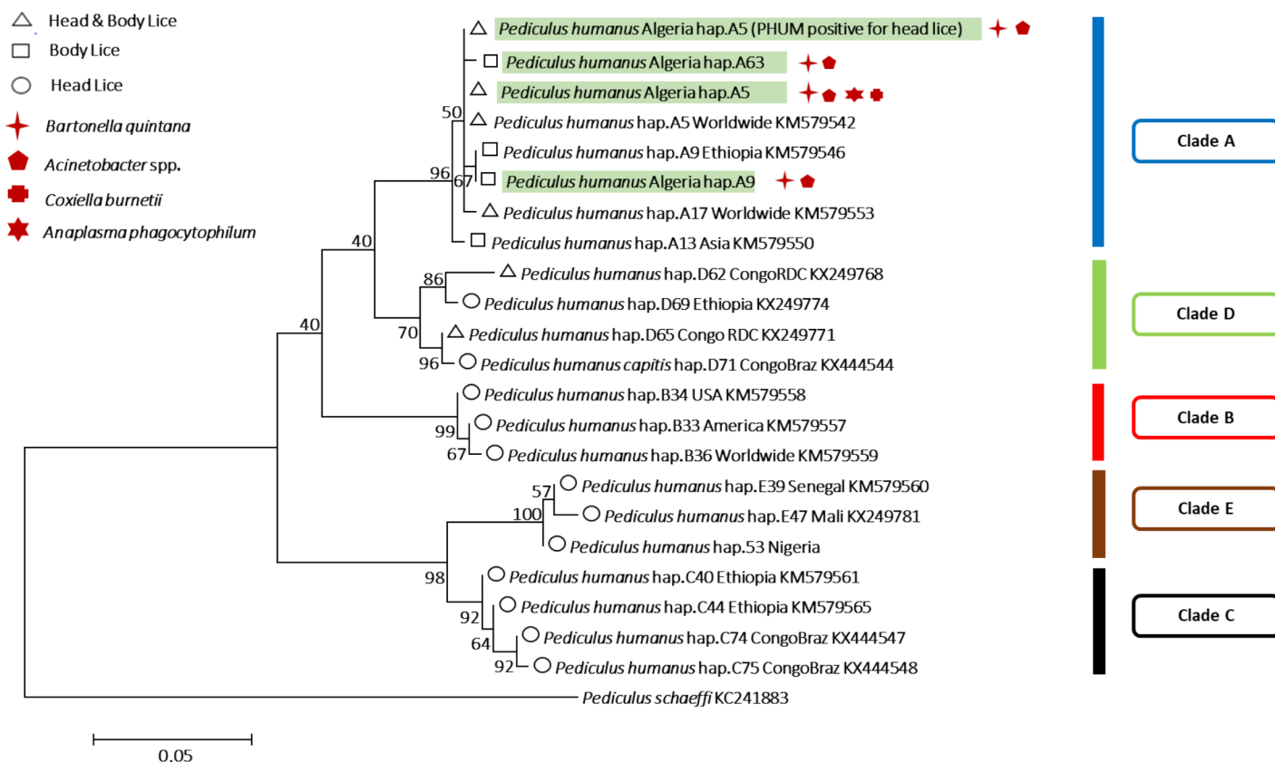
Fig 2. Phylogenetic tree showing the relationship of haplotypes identified in this study with other Pediculus humanus haplotypes. Phylogenetic inferences were conducted in MEGA 6 using the maximum likelihood method based on the Kimura 2-parameter. The GenBank accession numbers are indicated at the end. The mitochondrial clade memberships are indicated to the right of each tree. Specimens analyzed in this study are in green. A) Bacterial DNAs detected in body lice reported in this study. B) Lice samples positive for B. quintana , C. burnetii , A. phagocytophilum and Acinetobacter spp. and there are specified genotypes.
