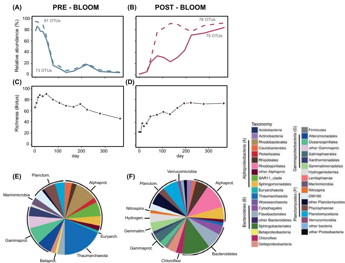
Fig. 4. Characteristics of the OTUs that displayed the largest changes in abundance during the experiment, i.e., 'responsive OTUs' (see text for details).
