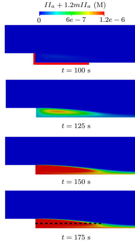
Fig. 8 Total thrombin concentration field at t = 100 , 125, 150 and 175 s. The black dashed line represents over which total thrombin is plotted in Fig. 9. The red line (at t = 100 ) represents approximately the experimental wall region of thrombus formation of Taylor et al. (2014).
