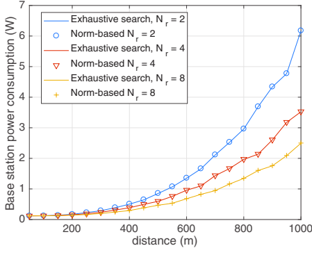
Figure 2. Comparison of NBS with an exhaustive search. With our simulation parameters, NBS provides optimal results.
