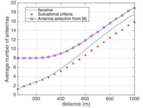
Figure 5. Comparison of the number of switched-on antennas with the proposed policy and with an exhaustive search.
