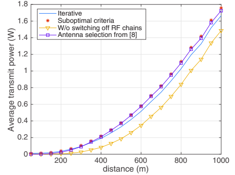
Figure 6. Comparison of the average transmit with the proposed policy, with the optimal ones and with the policy without switching-off antennas.
