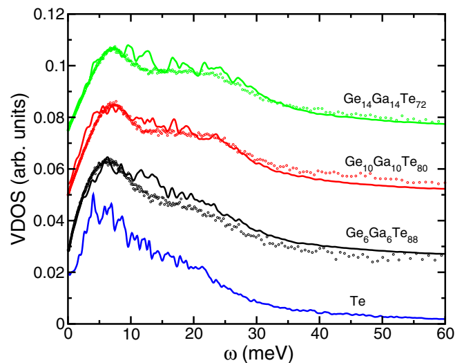
FIG. 12. Total measured (dots) and calculated (curves) vibrational density of states (VDOS) in \text{Ge}_x\text{Ga}_x\text{Te}_{100-2x} liquids. The VDOS of liquid Te has been added for comparison [23].
