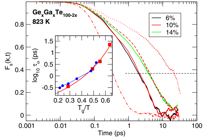
FIG. 15. Calculated Ga-based intermediate scattering function F_s(k, t) in Ge-Ga-Te liquids at 823 K. Additional red curves correspond to Ge 10 Ga 10 Te 80 liquids at 1500 K (dot-dashed), 773 K (broken), and 673 K (dotted). The horizontal line corresponds to 1/e and serves for the estimation of the relaxation time \tau_\alpha . The inset represents \tau_\alpha for Ge 10 Ga 10 Te 80 (red squares) in a reduced Angell plot where T_g has been taken as 428 K [11]. The red curve is a VFT fit [Eq. (8)] to the Ge-Ga-Te data using \log_{10} \tau_\infty = -13.12 and \mathcal{M} = 139 . Blue symbols correspond to data for Ge 2 Sb 2 Te 5 [14].
