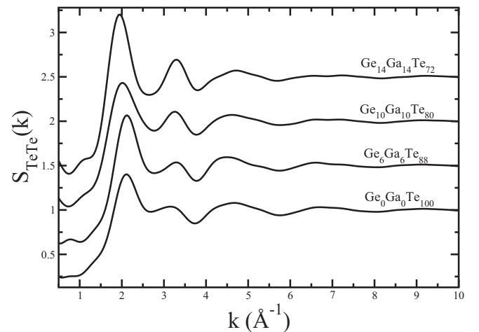
FIG. 8. Evolution of the simulated partial structure factor S_{\text{TeTe}}(k) with composition x in \text{Ge}_x\text{Ga}_x\text{Te}_{100-2x} at 823 K.
