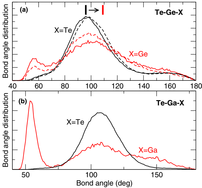
FIG. 11. Effect of homopolar bonds on the bond angle distributions Te-Ge-X (a) and Te-Ga-X (b) in \text{Ge}_{14}\text{Ga}_{14}\text{Te}_{72} liquids (823 K). (a) X=Te [same as Fig. 10(b)] or X=Ge (red curve). (b) X=Te [same as Fig. 10(c)] or X=Ga (red curve). In panel (a) are also represented corresponding results for \text{Ge}_{14}\text{Sb}_{14}\text{Te}_{72} [23] (broken curves). The arrow marks the shift of the average angle due to the presence of Ge-Ge homopolar bonds.
