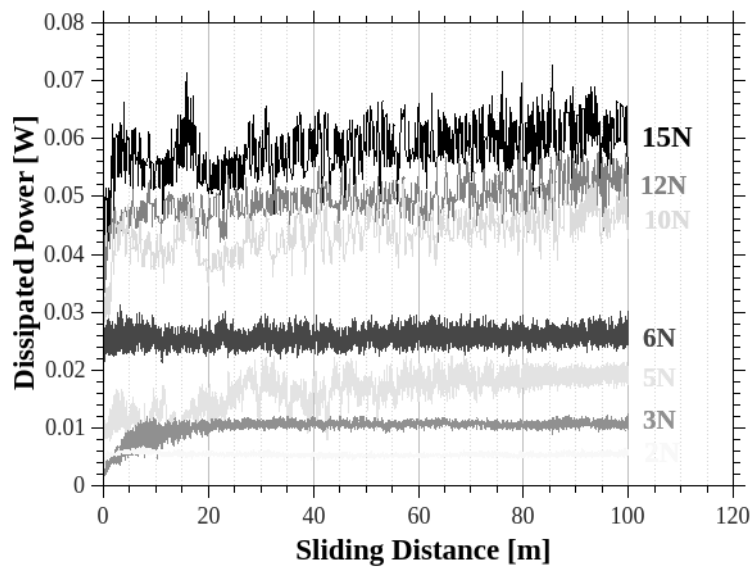
Figure 7: Variation of the dissipated power by friction vs. sliding length for various normal loads
