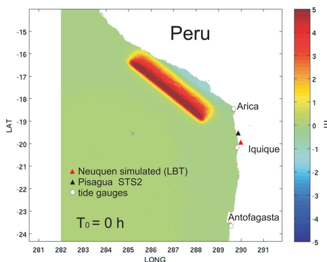
Figure 19. Model of tsunami for a M = 8.8 scenario earthquake in southern Peru. Sea level is plotted just after the seismic event (amplitude colour coded, in metres).
