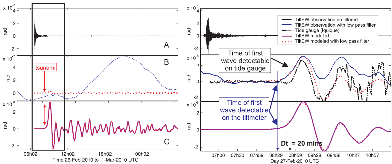
Figure 18. Early phase of STS2 observed and synthetic tilt at PSG for the 2010 Maule earthquake. (Left) 24 hr of signal; (right) zoom on the first 5 hr of signal. (a) EW tilt data computed from horizontal acceleration at PSG; (b) EW tilt at PSG, low pass filtered at 800 s (elliptic filter order 3), solid blue line shows the data, dotted red line is the synthetic computed from the tsunami model with the same filter; (c) synthetic EW tilt (same as red dotted line in (b), with enlarged vertical scale), unfiltered (solid purple line) and filtered (dotted red line) with the same filter as in (b). The rectangle in the figure to the left indicates the frame of the zoom on the right. Red and blue arrows point to the first signature of tsunami on tilt. Black arrow (right) points to the arrival time of tsunami on tide gauge (thin vertical black line).
