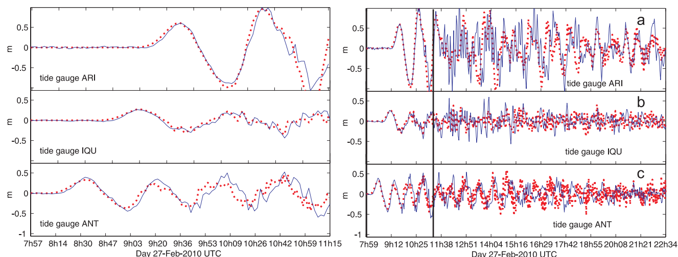
Figure 10. Tsunami records on three tide gauges for the 2010 Maule earthquake. Data (solid blue line) and synthetic (dotted red line) observed at the tidal gauges at Arica (a), Iquique (b) and Antofagasta (c). (Right) 15 hr of record; the vertical bar indicates the time segment shown on the left. The zoom shows the first 3 hr of tsunami.
