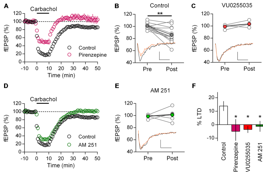
FIGURE 4 | Adult mice show M 1 mAChR dependent LTD in mPFC mediated by CB 1 R. (A) Time course of normalized field EPSPs in response to acute carbachol (10 μM, 10 min) stimulation in presence of M 1 mAChR antagonist pirenzepine (0.5 μM, n = 6 ; control, n = 14 ). (B) Individual experiments (gray) and group average, pre (baseline) and post (40 min washout) carbachol treatment (** P < 0.01 ). Below, example traces pre (black) and post (orange) carbachol treatment (scale bar: 5 ms, 0.1 mV). (C) Similar plot with highly selective M 1 mAChR antagonist VU0255035 treated group before (Pre) and after (Post) carbachol challenge; group averages in red (10 μM, n = 4 ). Below, example traces. (D) Time course showing normalized field EPSPs in response to carbachol stimulation in presence of CB 1 R antagonist AM251 (4 μM, n = 6 ). (E) Before-after carbachol challenge plot of individual experiments in presence of AM251, group average in green. Below, example traces. (F) Summary bar chart of percent LTD 40 min after carbachol washout (* P < 0.05 ).
