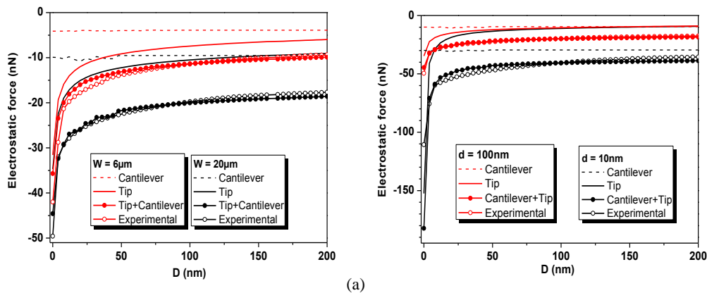
Figure 8. Comparison between simulated (tip + cantilever) and experimental EFDC (a) for various electrode width with a fixed electrode depth set to 100nm and (b) for various electrode depth with width set to 6\mu\text{m} . The
