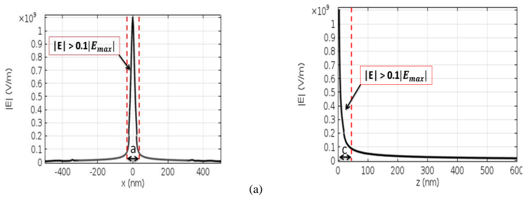
Figure 3. The electric field recorded (a) over the surface of the tip along the x-axis and (b) vertically between tip and sample surface along z-axis. D = 0\text{nm} , d = 100\text{nm} , W = 6\mu\text{m} and V_0 = 15\text{V} .
