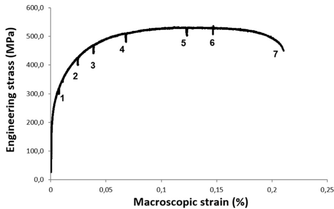
Fig. 4. Stress-strain curve recorded during in situ tensile testing in the SEM. 1–7 indicate the strain steps where the load is maintained and images are recorded.
