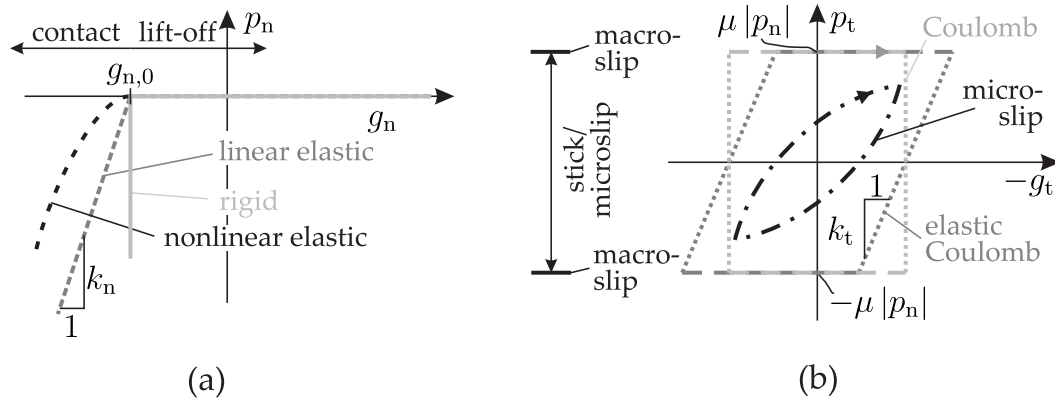
Fig. 7: Common contact laws: (a) unilateral laws for the normal contact, (b) friction laws for the tangential plane illustrated by their steady-state hysteresis for one-dimensional harmonic displacement and constant normal load
