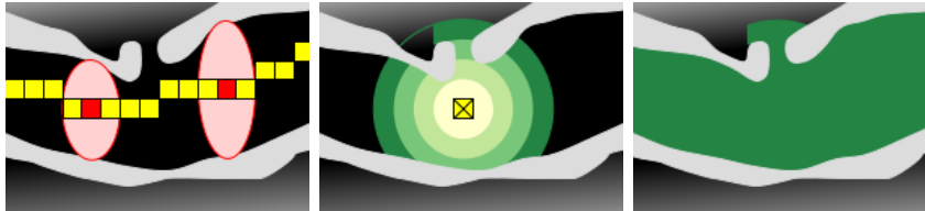
Fig. 2. Onion-kernel region-growing, (a) the input centerline tree is voxelized, (b) each centerline tree voxel becomes a seed; the segmentation is not allowed to grow backwards to fill the cavities (the dark green border delineates the region that would be filled otherwise), (c) the final segmentation.
