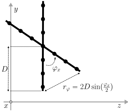
FIG. 2. Geometrical interpretation of l_\varphi with \varphi = \varphi_x . r_\varphi is the chord of \varphi , D is the radius of the microphone array (in black). Given D = 0.25 m, l_\varphi is set to be the maximum value of \varphi such that r_\varphi = 0.04 m.
