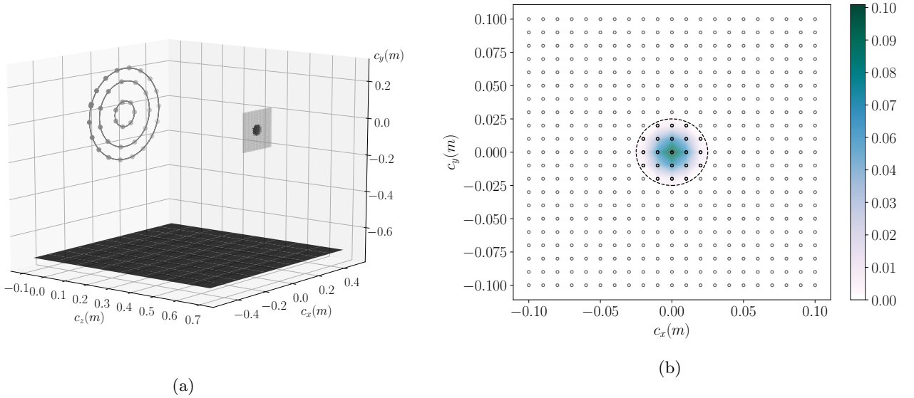
FIG. 1. (color online) (a) Scheme of the study case set-up including: the circular microphone array, the ground, and the reconstruction surface containing the acoustic source. (b) Colormap of the values characterizing the source strength. The dashed circle outlines the set of 21 monopoles (black dots) modeling the source. The nodes of the reconstruction surface are represented by the gray dots.
