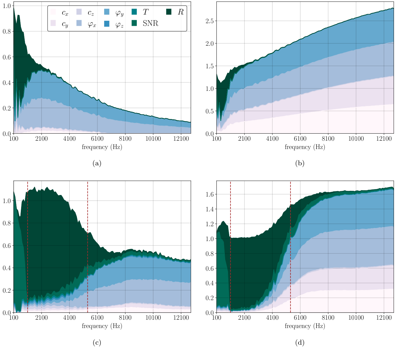
FIG. 4. (color online) Stack area charts for the MSE with Beamforming: (a) first-order Sobol' indices, (b) total effect Sobol' indices, and with Bayesian focusing: (c) first-order Sobol' indices, (d) total effect Sobol' indices.
