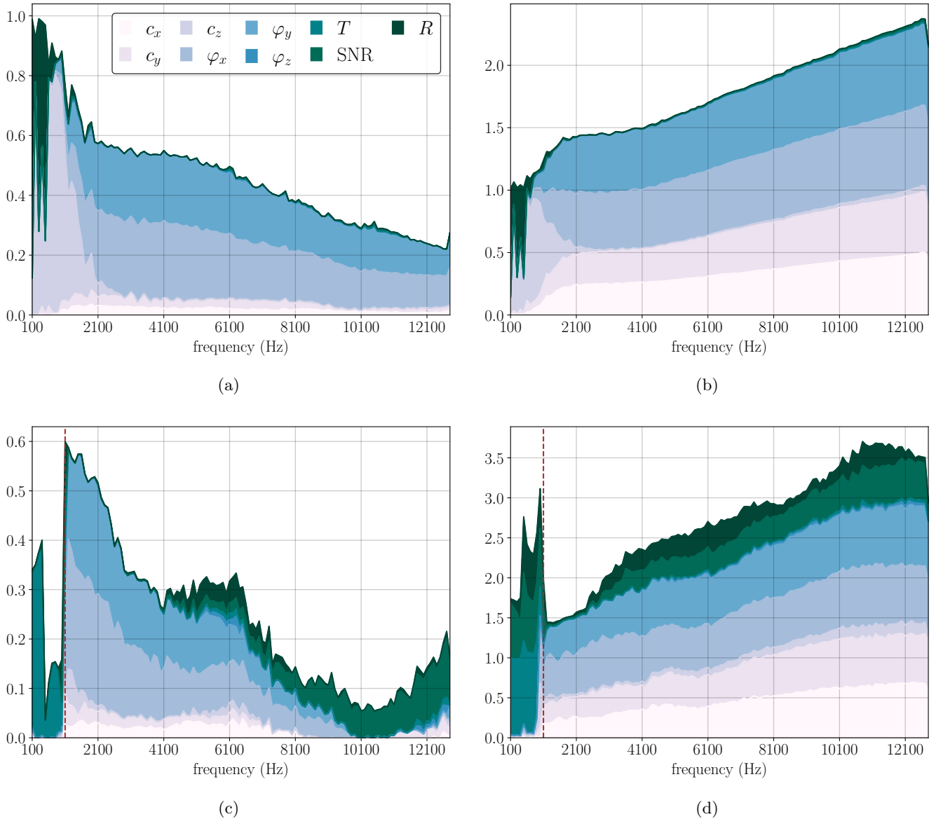
FIG. 5. (color online) Stack area charts for the acoustic power with Beamforming ( W_{beam} ): (a) first-order Sobol' indices, (b) total effect Sobol' indices, and with Bayesian focusing ( W_{baye} ): (c) first-order Sobol' indices, (d) total effect Sobol' indices.
