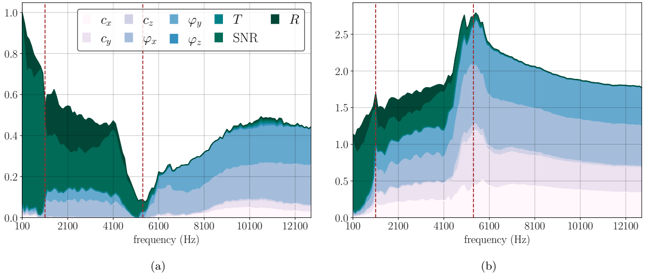
FIG. 3. (color online) Stack area charts for the regularization parameter \eta^2 . (a) First-order Sobol' indices. (b) Total effect Sobol' indices.
