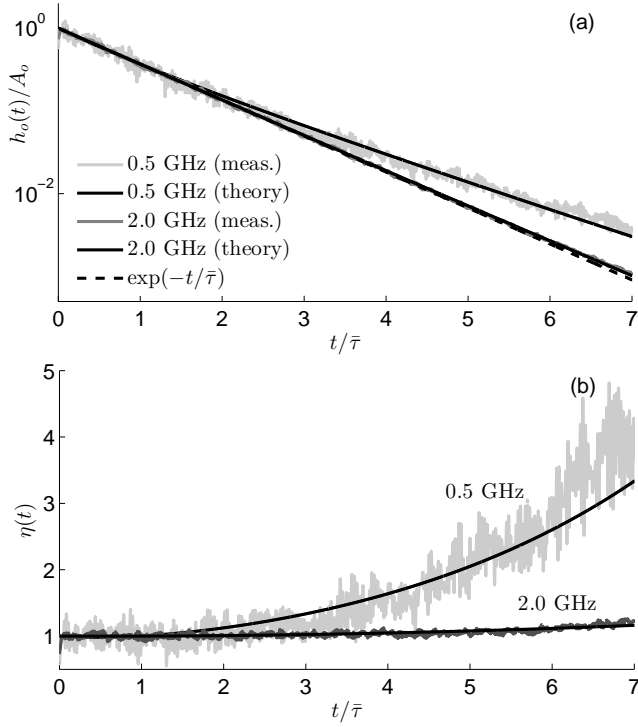
Figure 7: Validation results for the evolution of the IR envelope (i.e., the square root of the PDP) for B_T = 20 MHz, and f_c = 0.5 and 2 GHz, comparing experimental results (gray curves) and theory introduced in Sec. III (black curves), for : (a) the envelope and (b) the deviation function \eta(t, c) . Optimal fitting of theoretical results to experimental data yield an estimate of c = 0.34 (for f_c = 0.5 GHz) and c = 0.060 (for f_c = 2 GHz), corresponding to a relative standard deviation of 9.9 % and 1.7 % in the modal time constants \{\tau_k\} .
