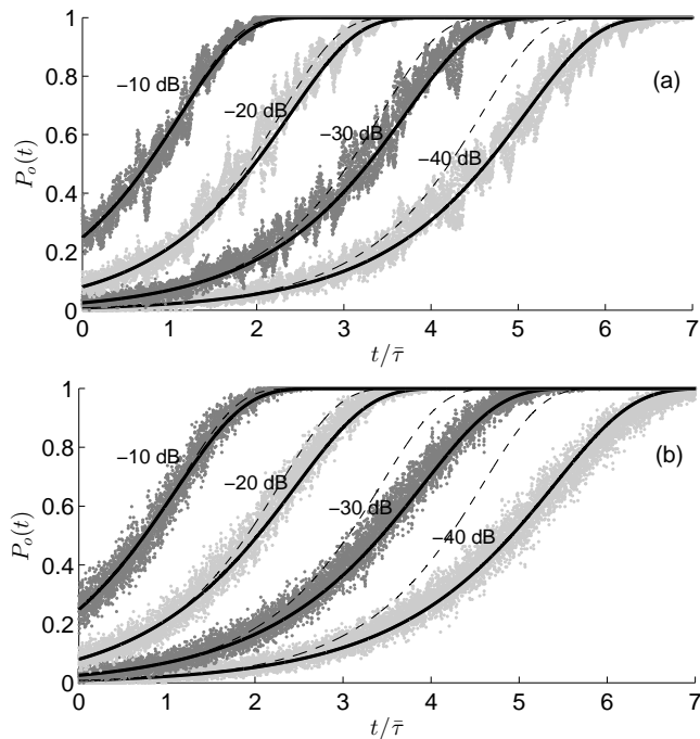
Figure 13: Empirical probability of receiving undetectable contributions, for four relative detection thresholds s_o , observed at 0.5 GHz, for: (a) B_T = 15 MHz and (b) B_T = 240 MHz. Local deviations in (a) are due to the limited number of DoF available and are consistent with those presented in Fig. 9. Theoretical predictions for a purely exponential IR envelope are shown as thin dashed curves, while solid thick curves take into account the correction \eta(t, c) introduced in (17).
