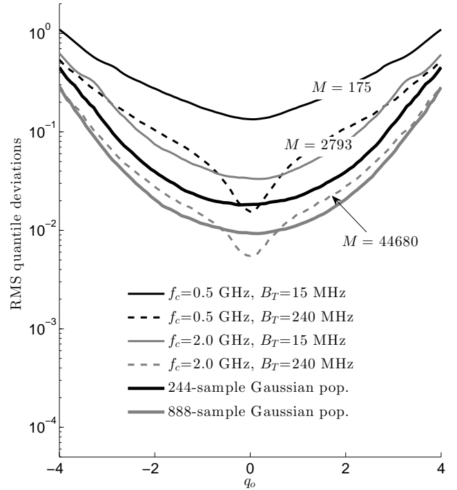
Figure 10: Comparison of the rms deviation between empirical and theoretical quantiles for w(t) , as a function of q_0 , for different choices of the excitation bandwidth and frequency. The number of modes available for each configuration is shown close to each curve. The two thicker curves represent the rms quantile deviation expected for ideally Gaussian-distributed populations, of sizes identical to those of the 0.5 GHz and 2 GHz datasets.
