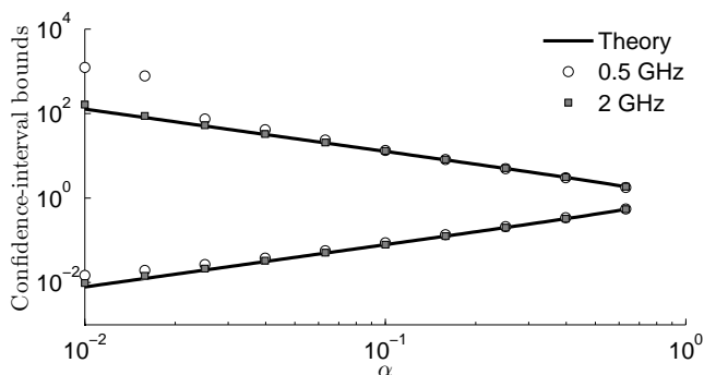
Figure 12: Bounds of the interval of confidence of the dynamic range spanned by |w(t + T_c)/w(t)| , for a varying significance level \alpha . Empirical results were obtained for B_T = 15 MHz and two central frequencies, spanning all time samples up to 7\bar{\tau} .
