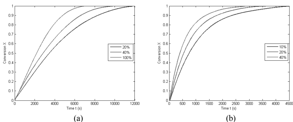
Figure 7. Influence of partial pressure of reacting gas on char conversion (a) under CO 2 atmosphere and (b) under H 2 O atmosphere (Temperature of reacting gas: 900°C)
