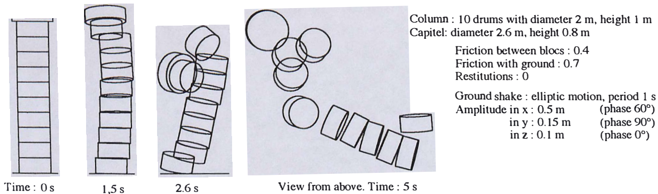
Figure 1: Column on shaken ground
