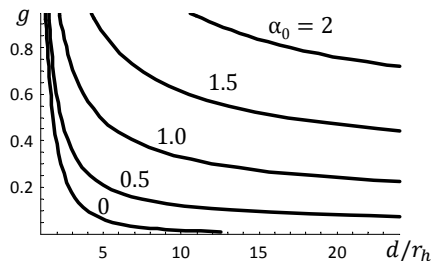
Figure 5. Dependence of the parameter g on the plasma flow divergence \alpha_0 and the ratio d/r_h according to Eq. (17). The values of \alpha_0 are shown with numbers near the correspondent curves.
