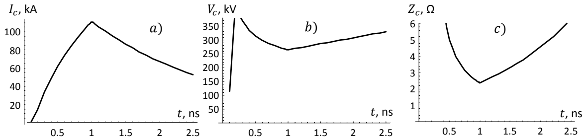
Figure 7. Temporal dependence of the current I_c (a) and tension (b) in the diode-coil circuit (a) and the circuit impedance Z_c = V_c/I_c (c). The parameters correspond to the experiment [8].
