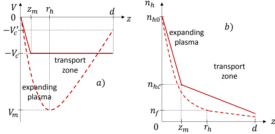
Figure 3. Potential (a) and density (b) distribution in the diode. Stationary distribution is shown with solid lines, dashed lines show the transient distribution before the potential equilibration.
