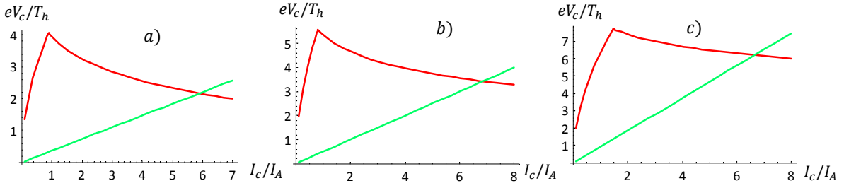
Figure 6. Current-voltage characteristic of the diode V_c(I) accounting for the effects of the space charge and magnetization. The chosen set of parameters corresponds to the experiments [5] a), [6] b) and [10] c). The distance between the diode plates is set to 1 mm and the resistance R_c = 1 \Omega
