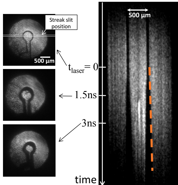
Figure 4. Optical shadowgraphy (at 532 nm) of the coil expansion. On the left, 0.65 ns-gated images corresponding to a cold coil (top, t = 0 ) and two different timings after laser-driving of the capacitor-coil target. On the right, the ns-scale expansion is resolved in a single shot by imaging the coil diameter into the slit of a streak camera. The average expansion velocity of the coil rod was measured to be 11 \pm 3 \mu\text{m/ns} (as indicated by the dashed orange line). Data acquired on the experimental campaign [8].
