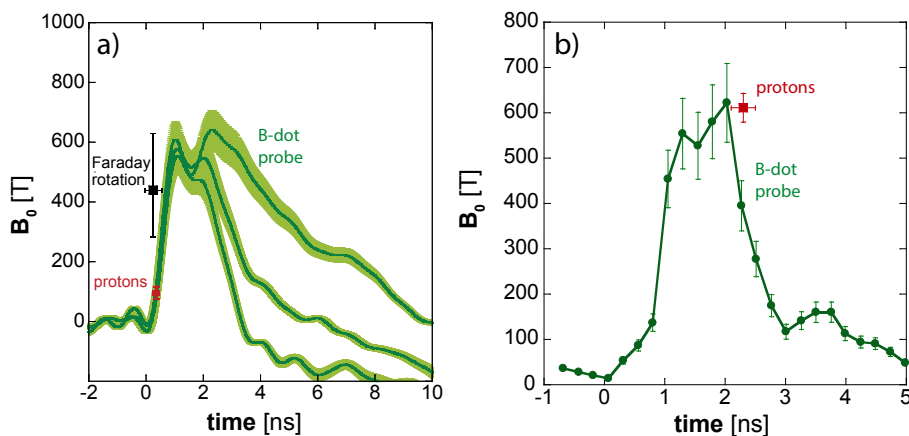
Figure 2. Measurements of magnetic fields at the coil center of nickel targets with different diagnostics as reported in Refs. [8] (a) and [9] (b).
