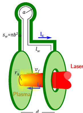
Figure 1. Scheme of the capacitor coil target with notations used in the paper. The materials commonly used for target fabrication are aluminum, copper, nickel and gold.
