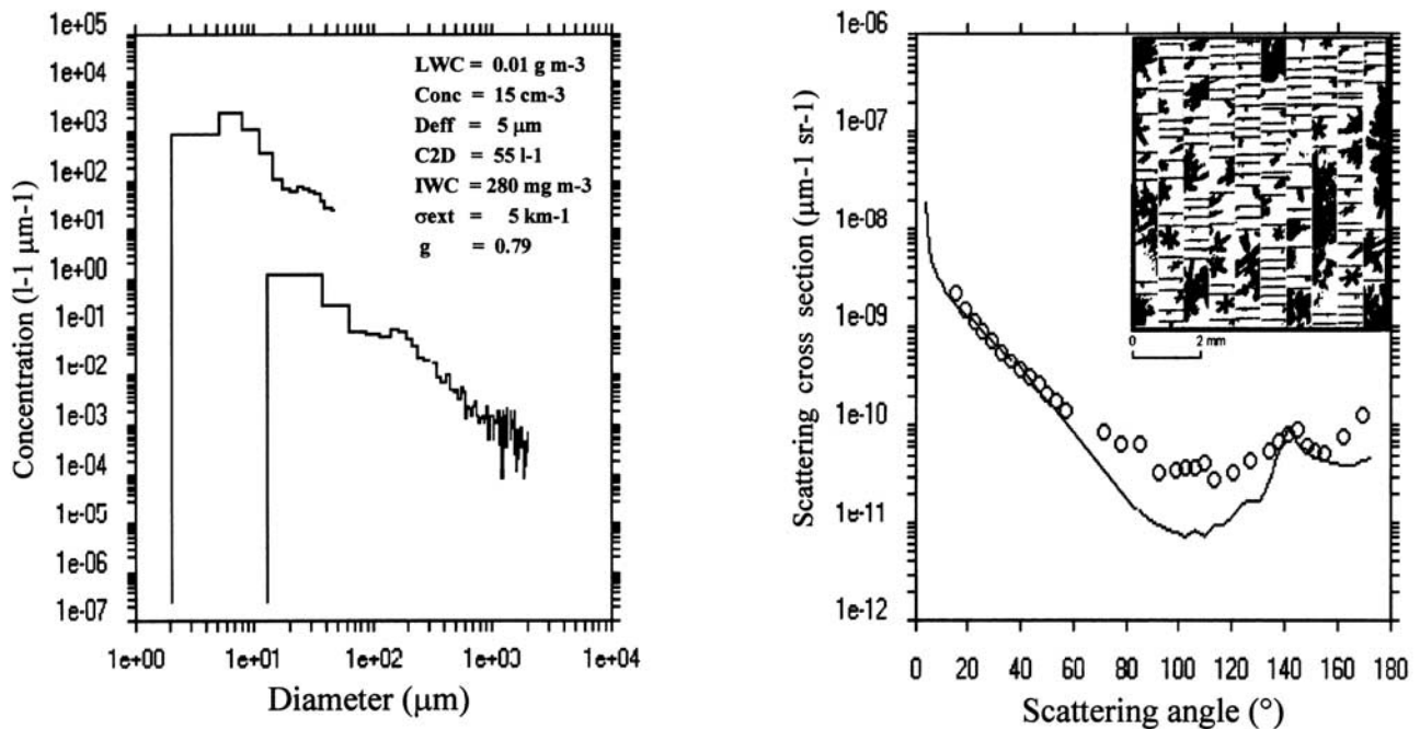
Figure 16. Same as Figure 15, but for data obtained near the cloud top at 2300 m (MSL) with a temperature of -15^{\circ}\text{C} during another 1 minute duration.
