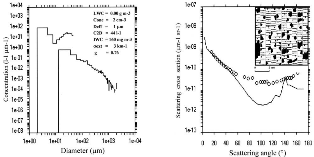
Figure 17. Same as Figure 15, but for data obtained in a precipitating region at 900 m (MSL) with a temperature of -6^{\circ}\text{C} during 1 minute duration.
