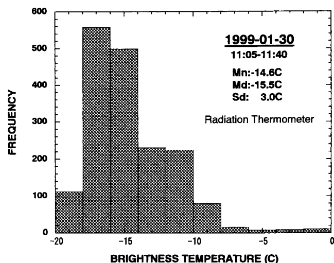
Figure 13. Histogram of the brightness temperature derived from nadir-looking infrared thermometer onboard the C404 for the stratocumulus cloud observed on 30 January 1999. Mn , Md and Sd are the mean value, the median value and the standard deviation, respectively.
