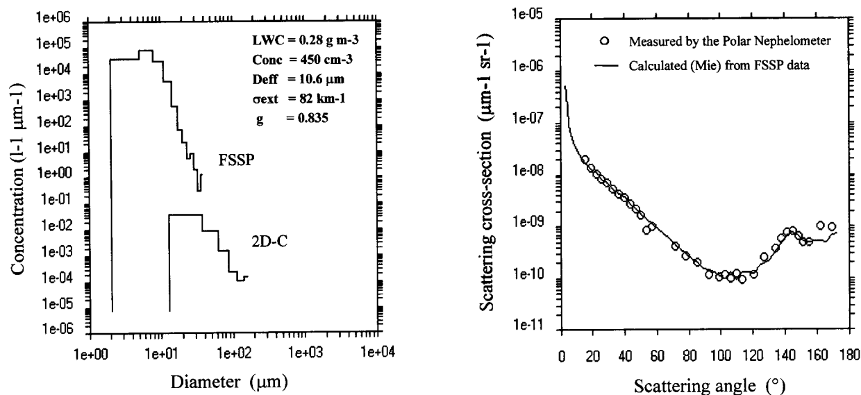
Figure 9. Same as Figure 2, but for the measurement near the cloud top at 1500 m (MSL) with a temperature of -6^{\circ}\text{C} . 21 January case study.
