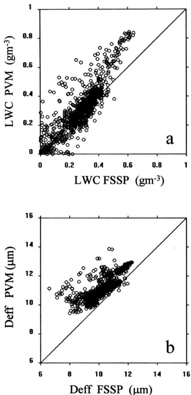
Figure 1. Comparison between Gerber PVM-100 and PMS FSSP probes for the stratocumulus cloud observed on 21 January 1999. (a) Liquid water content. (b) Effective diameter.
