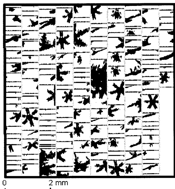
Figure 11. Example of ice particles sampled by the 2D-C probe near the cloud top at 2300 m (MSL) with a temperature of -15^{\circ}\text{C} for the stratocumulus cloud observed on 30 January 1999.
