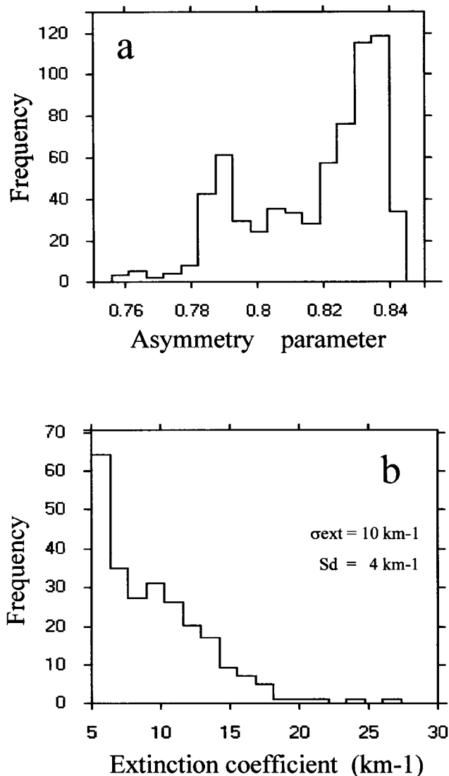
Figure 14. Frequency distributions of (a) asymmetry parameter and (b) extinction coefficient, measured near the cloud top for the stratocumulus cloud observed on 30 January 1999. The mean value and standard deviation are reported.
