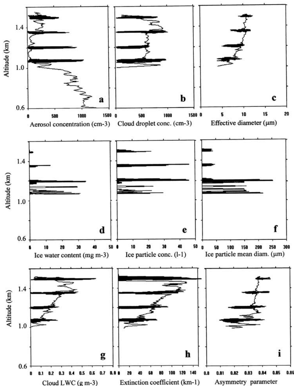
Figure 5. Vertical profiles of microphysical parameters relative to the 21 January stratocumulus case study: (a) aerosol concentration, (b) cloud droplet concentration, (c) effective diameter, (d) ice water content, (e) 2D-C particle concentration, (f) 2D-C mean particle diameter, (g) liquid water content, (h) extinction coefficient and (i) asymmetry parameter.
