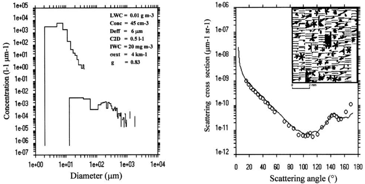
Figure 15. Example of measurements obtained by the Polar Nephelometer and the PMS FSSP and 2D-C probes. Data obtained near the cloud top at 2300 m (MSL) with a temperature of -15^{\circ}\text{C} during a 1 minute duration for the stratocumulus cloud observed on 30 January 1999. (left) Direct FSSP and 2D-C size-distributions (histogram representation) with values of the pertinent microphysical and optical parameters ( LWC , liquid water content; Conc , cloud droplet concentration; Deff , effective diameter; C2D , ice particle concentration; IWC , ice water content; \sigma_{ext} , extinction coefficient; g , asymmetry parameter). (right) Mean scattering phase function measured by the Polar Nephelometer (open circle symbols) and scattering phase function obtained by Mie theory (line) calculated with the average droplet size distribution measured by the FSSP over the same time period. An example of ice particle images sampled by the 2D-C probe is given in the upper right corner.
