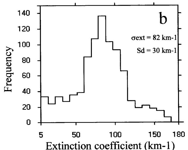
Figure 8. Frequency distributions measured near the cloud top of (a) asymmetry parameter and (b) extinction coefficient. The mean value and standard deviation are reported. 21 January case study.
