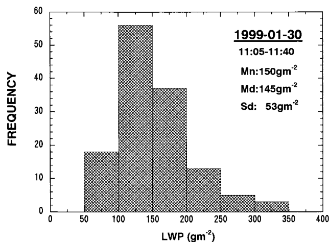
Figure 12. Histogram of the liquid water path ( LWP ) derived from nadir microwave radiance measurements (C404) for the stratocumulus cloud observed on 30 January 1999. Mn , Md and Sd are the mean value, the median value and the standard deviation, respectively.
