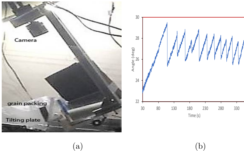
FIG. 1: (a) Experimental setup: view from the lateral camera: we can see the top camera moving with the tray, the pile of glass beads inside the small box with a white surface due to the light on top. The linear activator is on the back to permit the slow inclination. (b) Evolution of the surface of the grain packing obtained by an image analysis treatment of the white zone.
