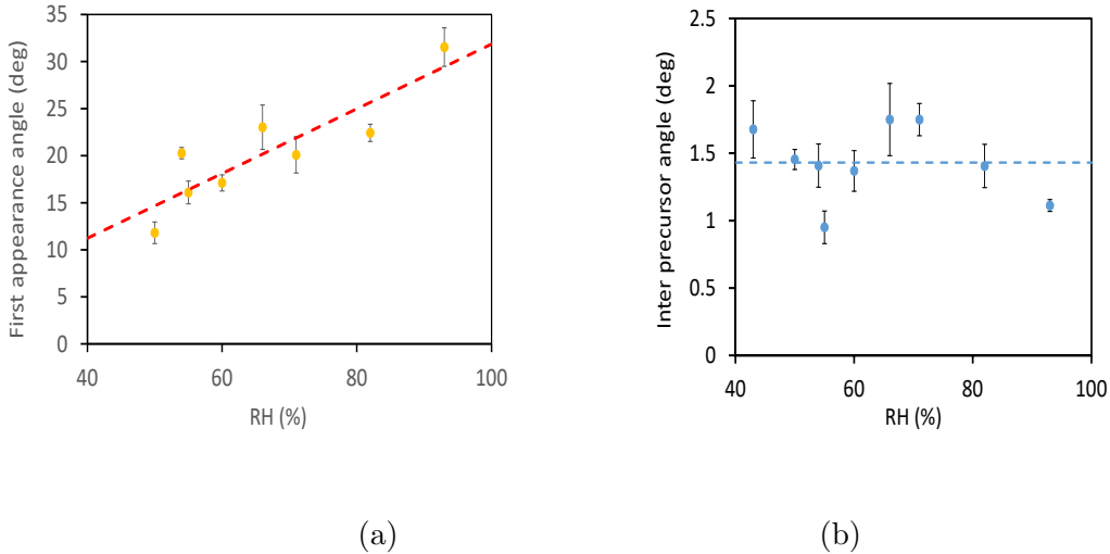
FIG. 8: Evolution of the appearance angle for the first precursor versus the humidity rate RH (a). Evolution of the inter-precursor angle versus the humidity rate RH (b).
