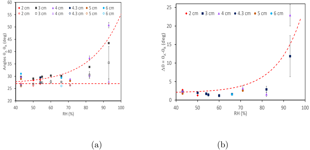
FIG. 7: Evolution of the maximum stability \theta_A (close symbols) and the repose \theta_R (open symbols) angles versus the humidity rate for the different available filling heights. The results are shown separately for each set of height H . The dashed lines are only guided lines for a better observation and have an exponential form for \theta_A .
