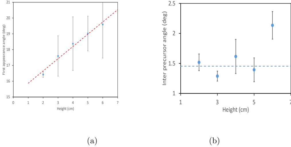
FIG. 6: (a) Appearance angle of the first precursor and (b) inter-precursor angle as a function of the pile height, measured for the experiments used in Figure 5. In (b) we have drawn an horizontal fit as we can assume that the H = 6\text{ cm} packing has a quite different packing history and cannot be compared directly to the other results.
