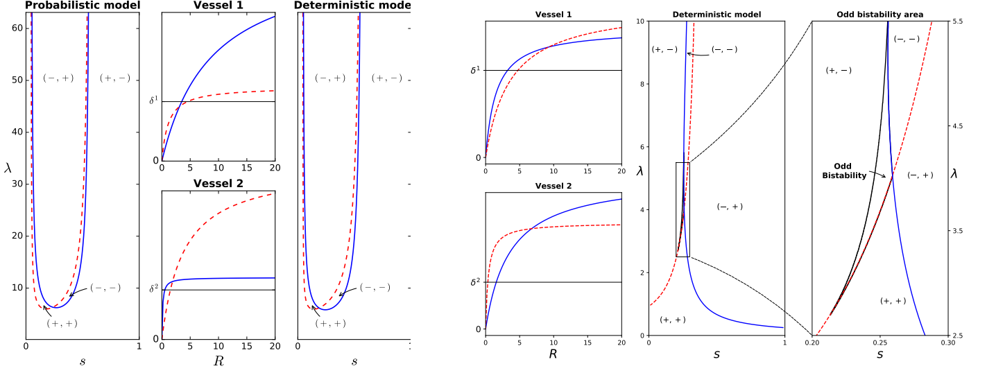
Figure 4: Two interesting situations. a - The two vessels are favorable to the same species. Depending on \lambda and s , each situation may occurs for both models (extinction of u or v , exclusive bistability or coexistence). (a_u^1, a_u^2, a_v^1, a_v^2) = (3.5, 2.5, 1.25, 7) , (b_u^1, b_u^2, b_v^1, b_v^2) = (8.75, 0.125, 1.125, 3.75) , (\delta^1, \delta^2) = (1, 2) and R_0 = 7 . b - A situation like in figure 3-a with an odd bistable area in the deterministic model (the probabilistic model behaves like the one figure 3-a). We show only the deterministic model and make a zoom on the odd bistable area in a (+, -) area. This zone corresponds to the case 3-(b) in the theorem 3.6. (a_u^1, a_u^2, a_v^1, a_v^2) = (3.7, 3.6, 4.4, 2.5) , (b_u^1, b_u^2, b_v^1, b_v^2) = (1.55, 3.55, 3.6, 0.4) , (\delta^1, \delta^2) = (2.5, 1.1) and R_0 = 20 .
