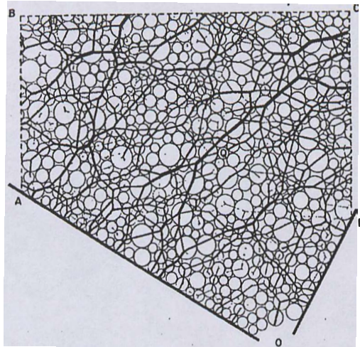
Figure 1: Contact forces in a sheared assembly of disks, visualized using the photoelastic effect, and encoded as widths of intercenter segments [Drescher and de Josselin de Jong, 1972].
