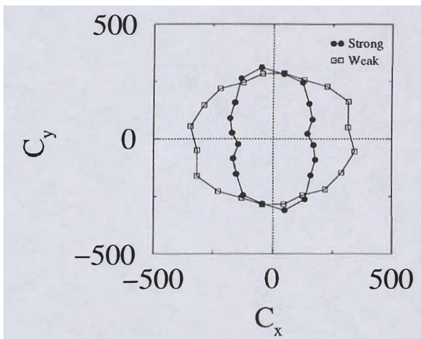
Figure 6: Polar diagram of the distribution of contact orientations in weak and strong subnetworks.
