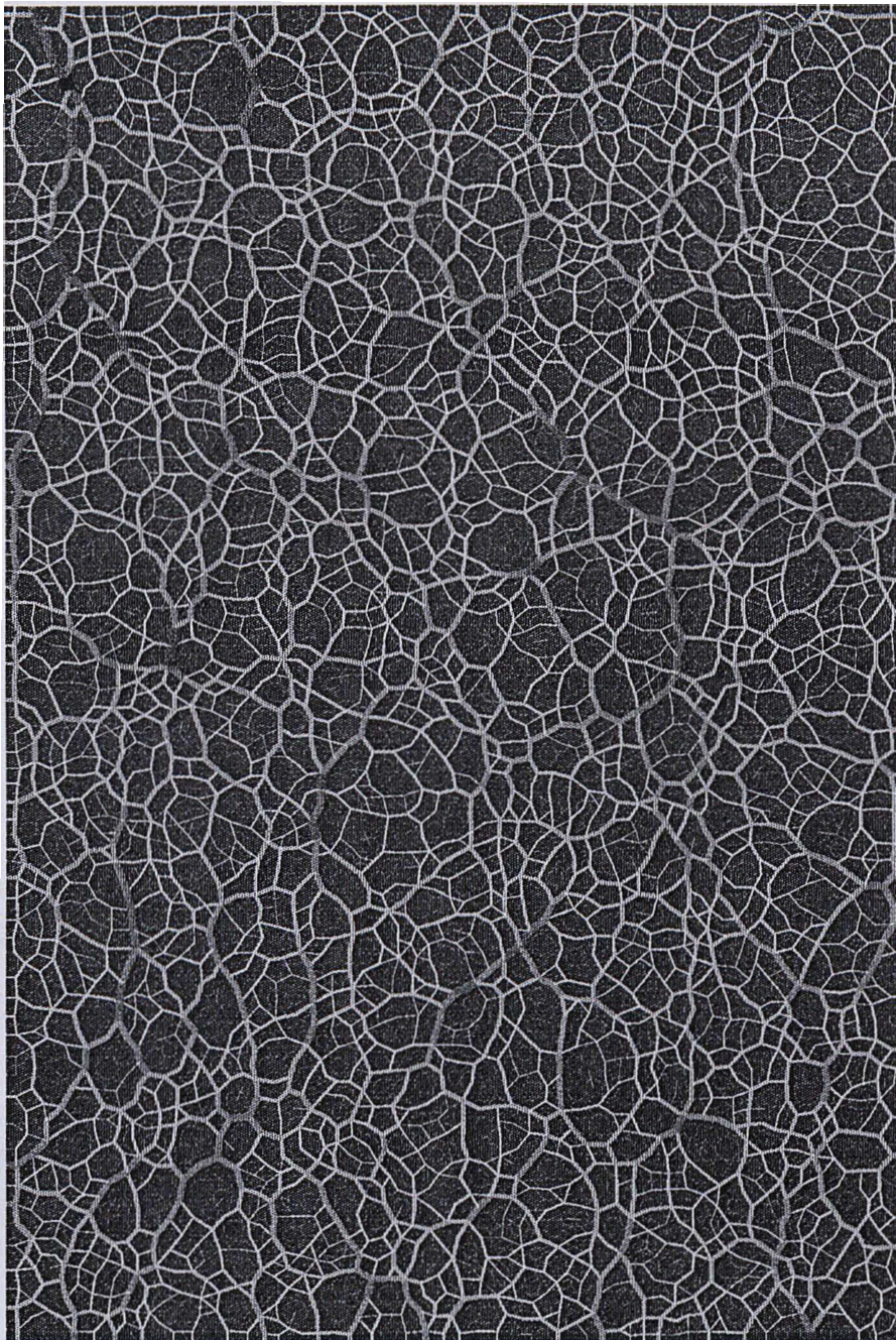
Figure 2: Normal components of the contact forces in sample A (see text) encoded both as the widths of intercenter connecting segments and by the color intensity.
