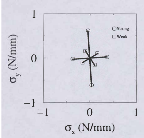
Figure 5: Contributions of weak and strong contacts to the stress tensor in sample A at shear peak.
