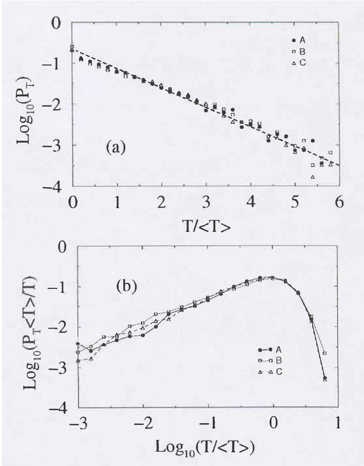
Figure 4: (a) Semilogarithmic, and (b) log-log plots of the probability distribution P_T of friction forces T .
