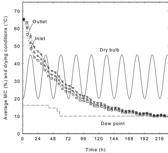
Fig.5. Evolution of drying conditions at the stack inlet and MC evolution of identical boards of the same layer (Configuration B)
