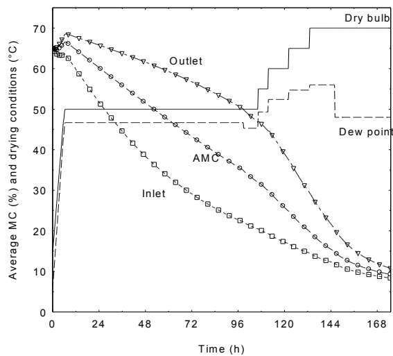
Fig.2. Evolution of drying conditions at the stack inlet and MC evolution of identical boards of the same layer (Reference configuration)
