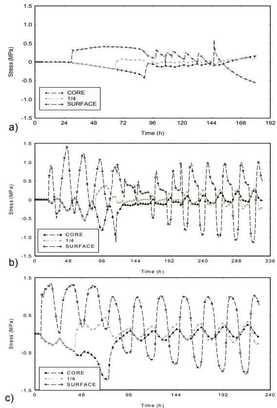
Fig.8. Drying stress within the board dried with the reference schedule (a), the strategy A (b) and B (c). Board is located at the stack inlet.
