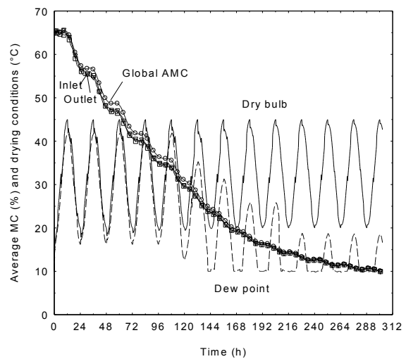
Fig.4. Evolution of drying conditions at the stack inlet and MC evolution of identical boards of the same layer (Configuration A.bis)
