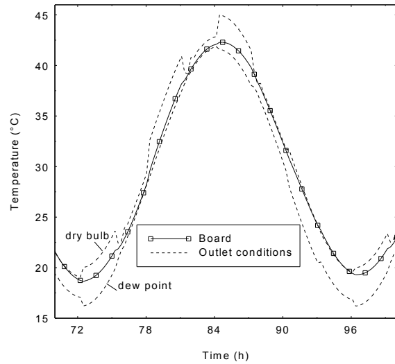
Fig.7. Enlargement on one period of the drying conditions and the surface temperature close to the stack outlet (Configuration A.bis)
