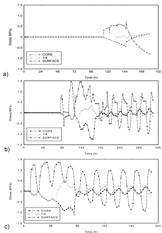
Fig.8. Drying stress within the board dried with the reference schedule (a), the strategy A (b) and B (c). Board is located at the stack inlet.
