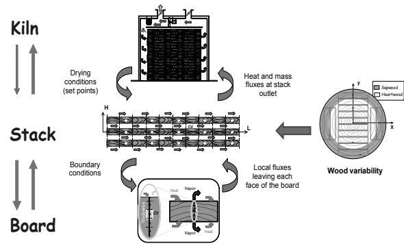
Fig. 1. Structure of the multiscale approach applied in the present work for the drying of a whole stack of boards.
