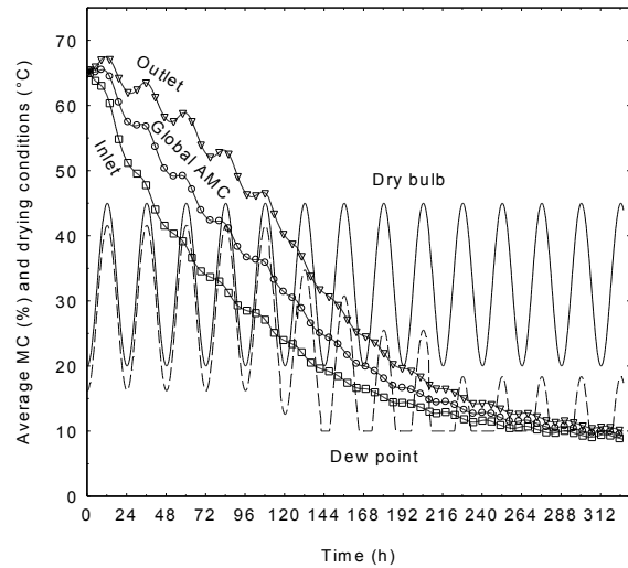
Fig.3. Evolution of drying conditions at the stack inlet and MC evolution of identical boards of the same layer (Configuration A).
