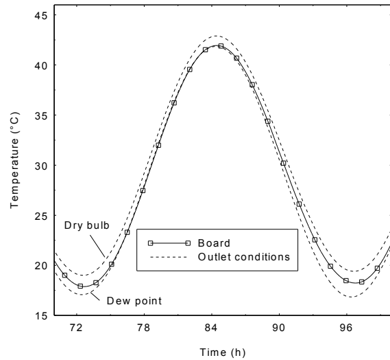
Fig.6. Enlargement on one period of the drying conditions and the surface temperature close to the stack outlet (Configuration A).
