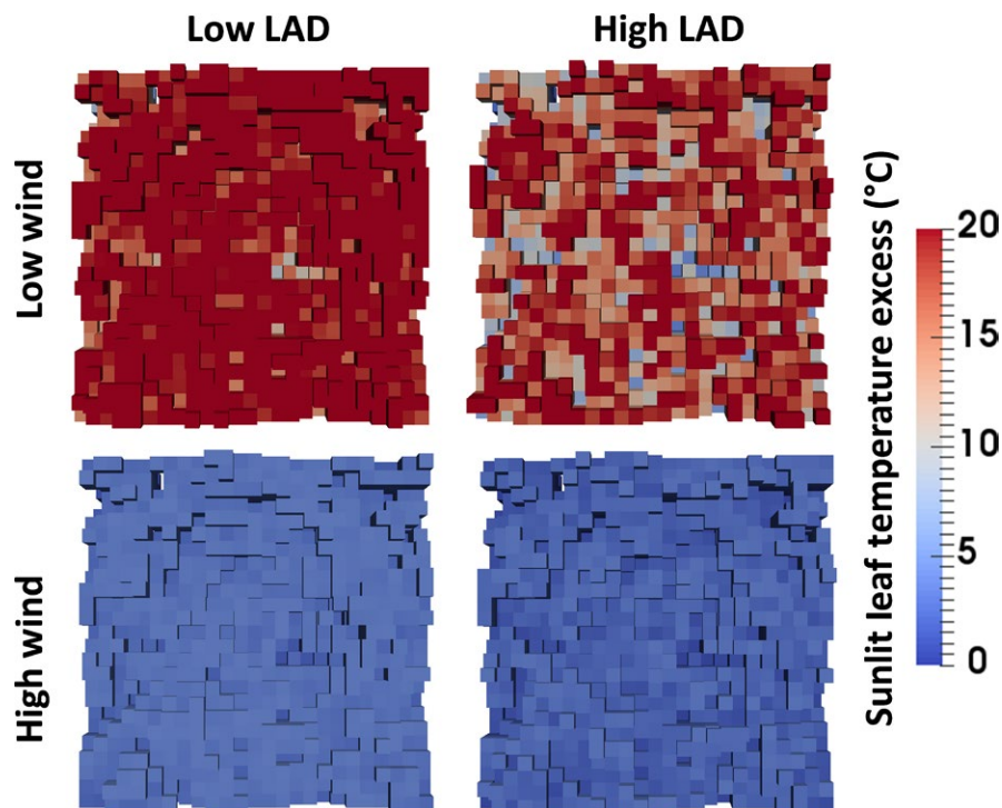
FIGURE 2 Two-dimensional presentation of the spatial distribution of sunlit leaf temperature excess (i.e., leaf temperature minus air temperature) for top view voxels in a portion of the continuous canopy (i.e., when the canopy is viewed from above). In this example, four different simulations are shown, under low and high wind speed (0 and 5 m/s) factored with low and high leaf area density (LAD, 2.36 and 9.46 m 2 /m 3 ). Colors refer to the amplitude of the sunlit leaf temperature excess. The voxels appearing in white correspond to gaps in the canopy, through which the ground can be seen from above the canopy. In all simulations, the other parameters were fixed: irradiance = 1,200 W/m 2 ; air temperature = 20 °C; Kt = 0; G max = 0.004 m/s
