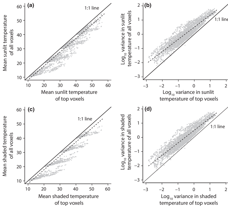
FIGURE 6 Regression analysis of mean temperature and variance of all voxels in the continuous canopy as a function of top-viewed voxels for both sunlit (a, b) and shaded (c, d) portions of voxels. Color-coded versions of these figures are available in Appendices S4–S7, which show the effects of four other main variables ( T_{\text{air}} , wind, irradiance, and LAD) on these relationships (Figure 6a, linear regression: p < .001 , R^2 = .95 , y = 0.97x - 1.62 ; Figure 6b: p < .001 , R^2 = .87 , y = 0.87x + 0.50 ; Figure 6c: p < .001 , y = 0.98x - 1.75 ; Figure 6d: p < .001 , R^2 = .87 , y = 0.87x + 0.48 )
