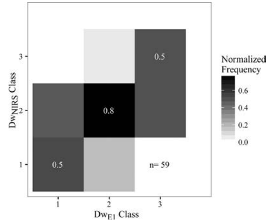
Fig. 12. Contingency table of Dw_{E1} and Dw_{NIRS} classes.
