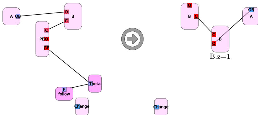
Fig. 10. Follow Decision. Transfers asset and prepares for a new transaction (i.e. cleans up after the decision to follow the negligence rule), setting buyer’s attribute z to 1 (which indicates negligent behaviour) and increasing the Change counter sumofchange if there was a change in the bank’s behaviour (i.e., if the new value of z is different from PB’s value).
