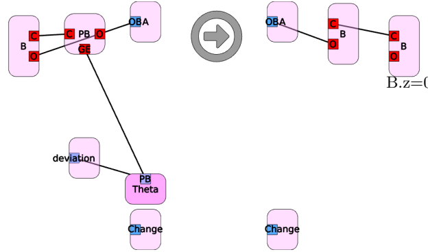
Fig. 12. Deviation Decision. Transfers asset and prepares for a new transaction (i.e. cleans up after the decision to deviate from the negligence rule), setting buyer's attribute z to 0, and increasing the Change counter sumofchange if there was a change in the bank's behaviour (i.e., if the new value of z is different from PB's value).
