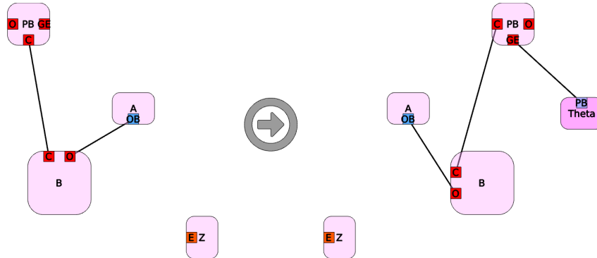
Fig. 8. Begin Analysis. Computes profitability U1, U0 of PB, generating a node Theta with attribute \Delta U1U0 = U1 - U0
