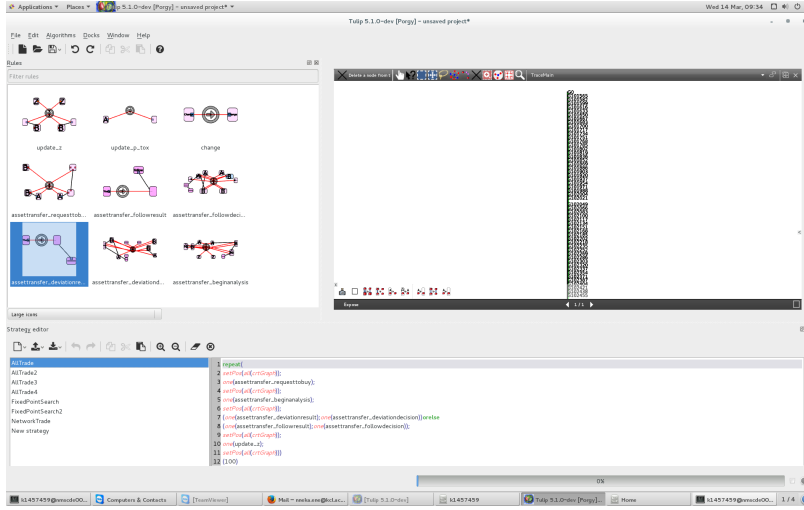
Fig. 4. PORGY in action: A portion of a branch in a derivation tree (top right window). Bottom window: strategy widget, left window: rules widget containing all the rules that drive the system. The diagram has been minimized in keeping with space restrictions. A zoom-in on the derivation tree can be found in Figure 5. Sample strategies can be seen in Section 3.
