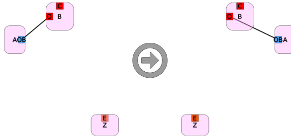
Fig. 13. Update Z. Updates the attribute z in node Z (which represents the average of the values of z in each bank). The new value in Z is (Z * (k - 1) + z(PB)) / k
