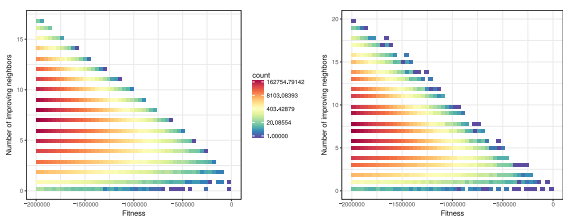
Figure 5: Correlation between fitness and the number of improving neighbors with color in log scale. 2ckx (left), and 2gkt (right).
