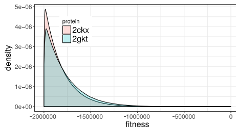
Figure 1: Density of states over fitness.
