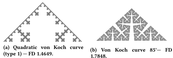
Figure 1: Two fractals, both with dimensions between one and two.
