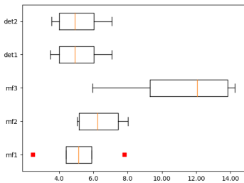
(b) Fractal dimensions of the LONs extracted from benchmark QAP instances ( Nug group).
