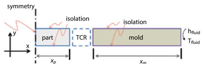
Figure 3 One-dimensional heat transfer problem in the thickness direction x .
