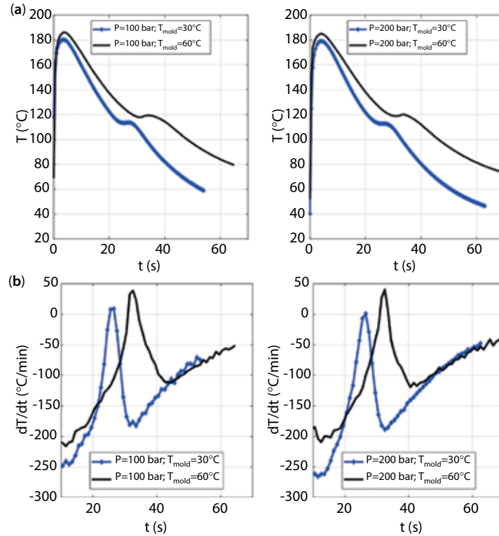
Figure 4 Flying probe temperature measurements: (a) T(t) curves and (b) their time derivative dT(t)/dt curves obtained for two holding pressures (100 and 200 bars) and two mold temperatures 30 and 60 °C.
