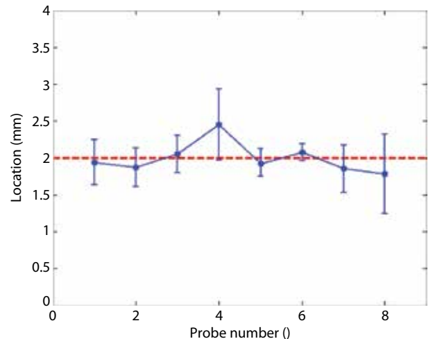
Figure 2 Distribution of flying temperature probe thermocouple positions for the different injected samples (location around 2 mm, in the center of the mold cavity).
