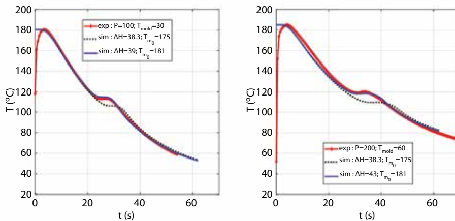
Figure 5 Simulations vs. experimental data for two sets of molding conditions (pressure, temperature and enthalpy of crystallization are given in bar, °C and kJ/kg, respectively).
