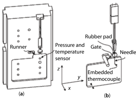
Figure 1 Instrumented molding cavity (a) and flying temperature probe (b).
