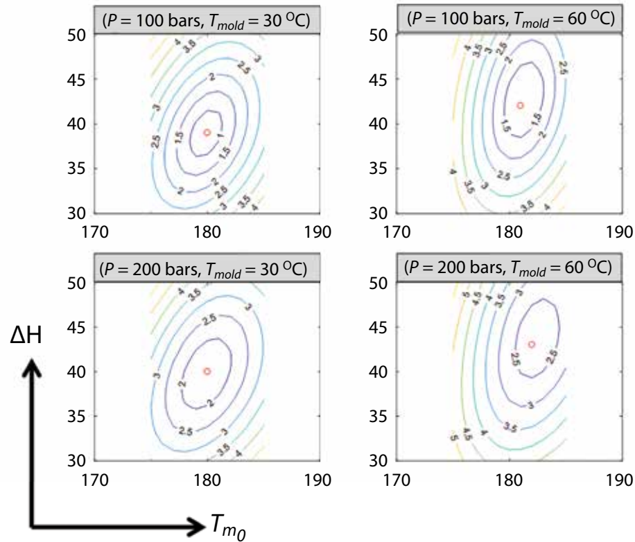
Figure 6 Influence of \Delta H and T_{m0} values on absolute mean square difference between simulated and measured temperature curves for four molding conditions.
