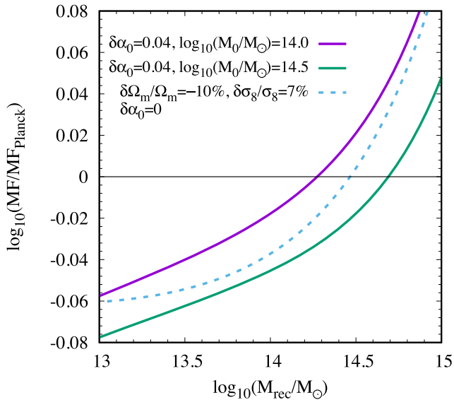
Figure 9. The impact of neglecting the flattening of the M_{\text{rec}}-M_{\text{true}} relation due to mass-dependent imperfect membership on the observationally measured mass function (MF). It is assumed that the M_{\text{rec}} \propto M_{\text{true}}^{\alpha_0} relation is determined in a very narrow mass range about M_0 , leading to a bias \delta\alpha_0 when extrapolating the relation to lower and higher masses. The dashed line shows the mass function for modifications of cosmological parameters that approximately compensate the effects of mass-dependent imperfect membership. The mass functions are calculated relative to a fiducial model given by the Planck cosmology ( \text{MF}_{\text{Planck}} ).
