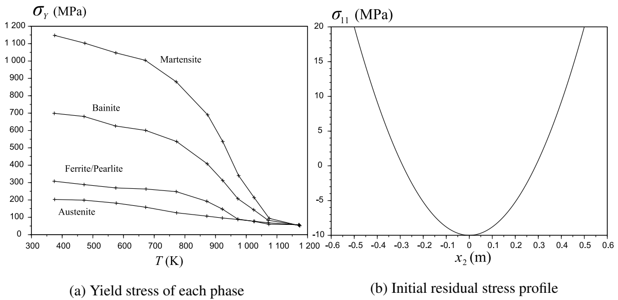
Figure 7: Coupled thermal/metallurgical problem
