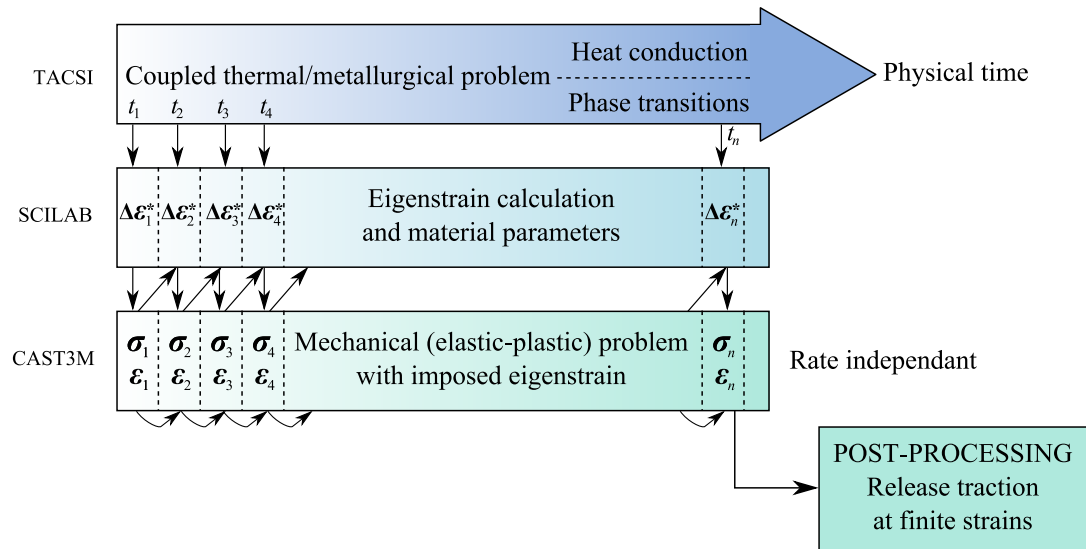
Figure 3: Numerical scheme
