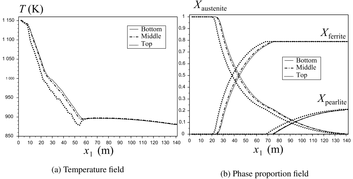
Figure 7: Coupled thermal/metallurgical problem
