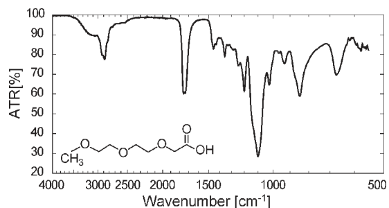
Figure 13. Infrared spectra of MEEAA recorded on a spectrum 100 FTIR with a universal ATR sampling accessory.
