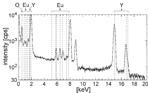
Figure 7. Energy-dispersive X-ray spectrum measured on the TEM picture (Figure 2d) corresponding to the \text{Y}_2\text{O}_3 synthesis performed using the complexing molecule (#2). The atomic percents are deduced from spectra measured at different positions on the TEM sample. The percentages are 56.5 \pm 12.0 at. % of C, 43.3 \pm 12.1 at. % of O, 0.18 ± 0.06 at. % of Y, and 0.02 \pm 0.01 at. % of Eu.
