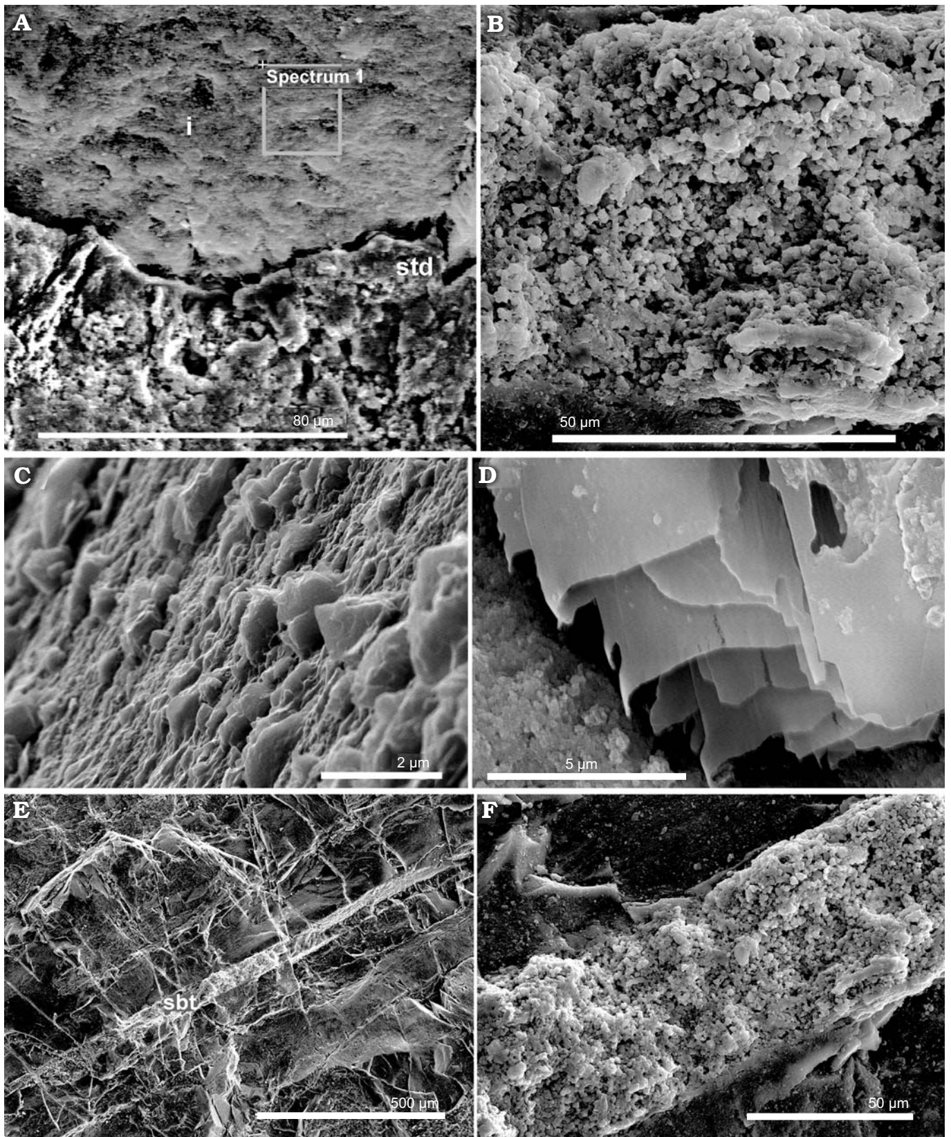
Fig. 9. Coleoid cephalopod Idahoteuthis parisiana Doguzhaeva and Brayard gen. et sp. nov. (holotype, UBGD 30545); middle Olenekian, Early Triassic; Idaho, USA; globular ultrastructure of non-biomineralized structures. A. Sheet-like patch of flooded ink (top) and soft tissue debris (bottom); a site of the geochemical analysis is marked with a square. B. Undetermined long soft tissue piece showing a micro-granular ultrastructure on the dorsal side of the soft body. C. Micro-laminated ultrastructure of the gladius. D. Undetermined non-biomineralized micro-laminated fragment from the stomach. E. A linear fragment of soft tissue on dorsal side of the body. F. Micro-globular ultrastructure. Abbreviations: i, ink sheet-like patch; sbt, soft body tissues; std, soft tissue debris.
