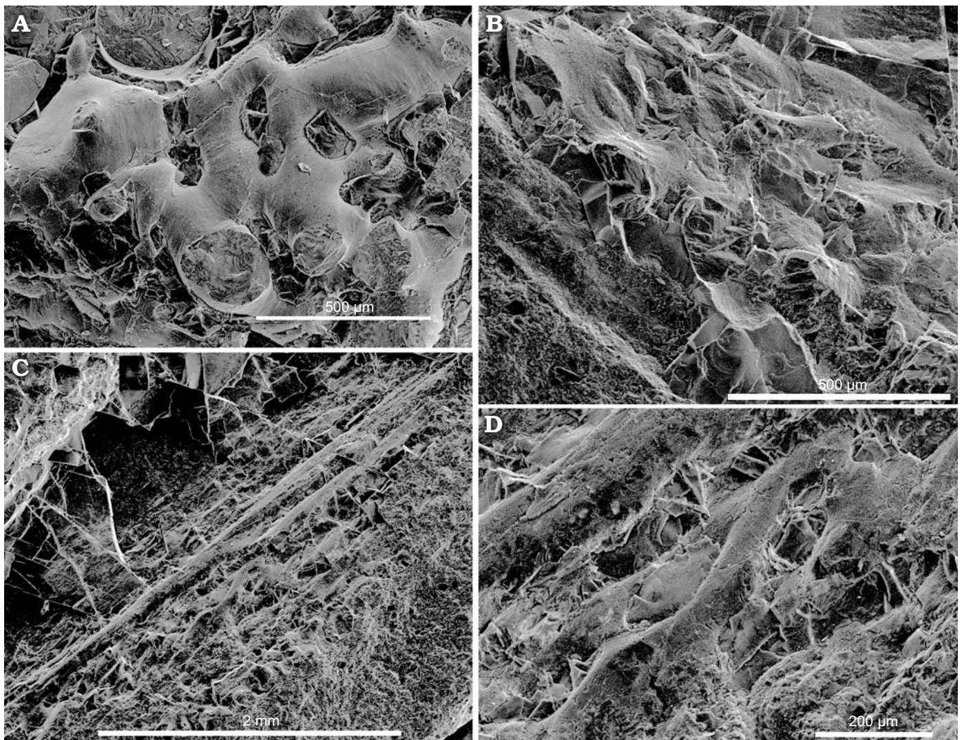
Fig. 8. Coleoid cephalopod Idahoteuthis parisiiana Doguzhaeva and Brayard gen. et sp. nov. (holotype, UBGD 30545); middle Olenekian, Early Triassic; Idaho, USA. A . Canalicular cartilage of fin-supported structure. B–D . Cartilaginous mantle band-shape structure on dorsal side showing a canalicular type of cartilage.
