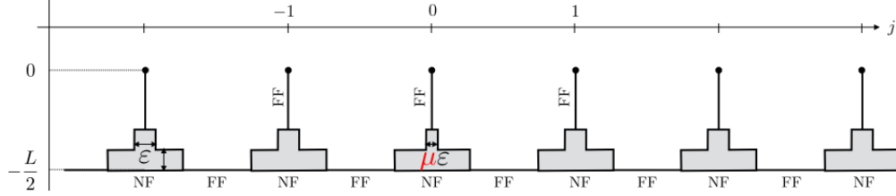
Figure 5: Schematic representation of the asymptotic expansion (NF: near field, FF: far field)
