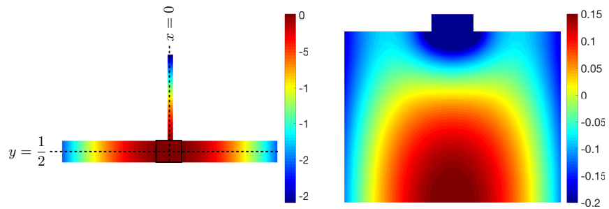
Figure 16: the near field terms U_0^{(2)}
