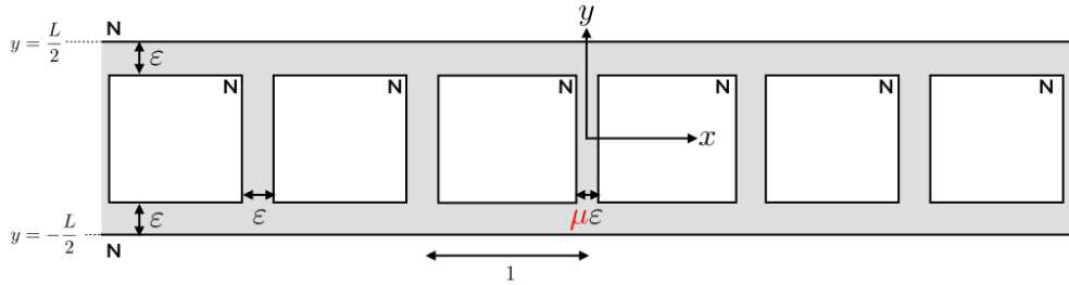
Figure 2: The Perturbed ladder
