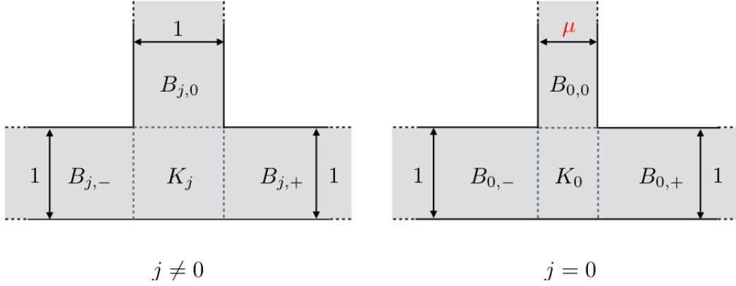
Figure 6: The junctions \mathcal{J}_j (perturbed for j = 0 and unperturbed for j \neq 0 )
