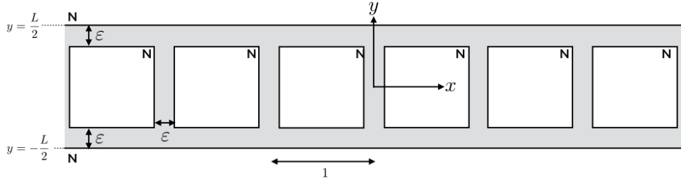
Figure 1: The unperturbed periodic ladder
