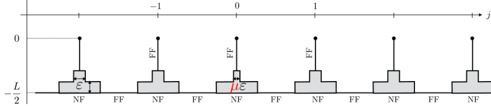
Figure 5: Schematic representation of the asymptotic expansion (NF: near field, FF: far field)
