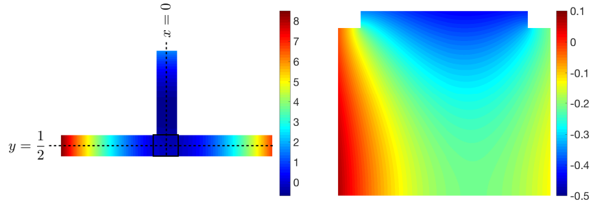
Figure 19: the near field terms U_1^{(2)}
