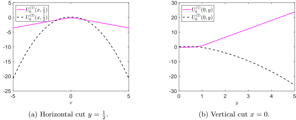
Figure 17: Representative curves of the near fields U_0^{(1)} and U_0^{(2)} along the cuts y = \frac{1}{2} and x = 0 in \mathcal{J}_0
