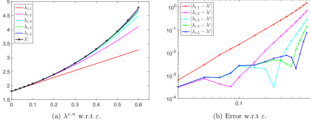
Figure 12: Results for the first eigenvalue.
