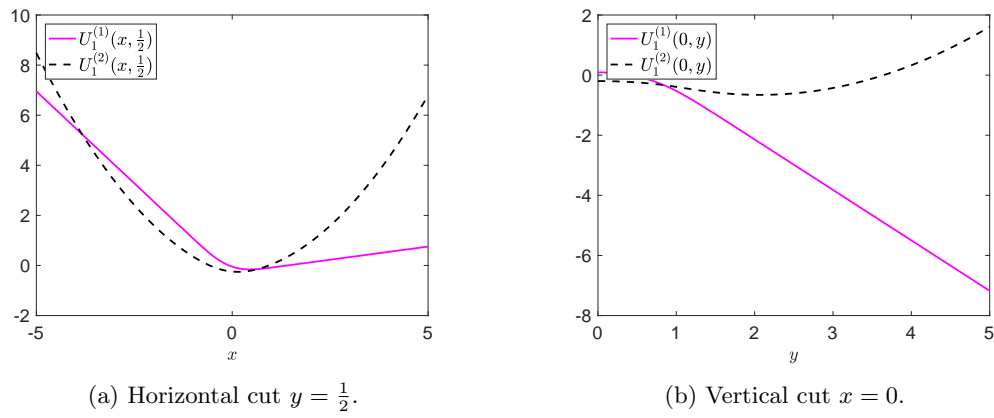
Figure 20: Representative curves of U_1^{(1)} and U_1^{(2)} along the cuts y = \frac{1}{2} and x = 0 in \mathcal{J}_1
