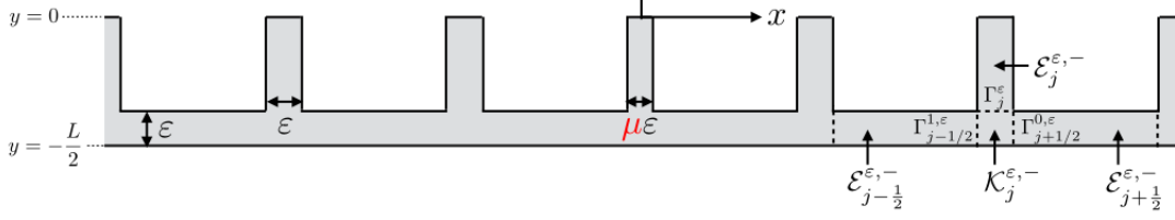
Figure 4: The domain \Omega_\varepsilon^{\mu, -}
