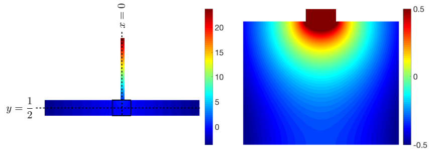
Figure 15: the near field terms U_0^{(1)} (right part: zoom of the area inside the black rectangle)
