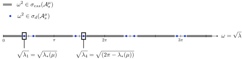
Figure 10: The spectrum of \sigma(\mathcal{A}_s^\mu) in the case L = 2 .
