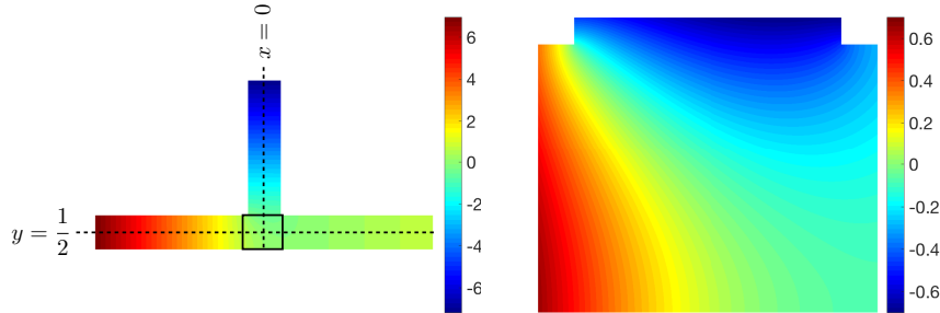
Figure 18: the near field terms U_1^{(1)}
