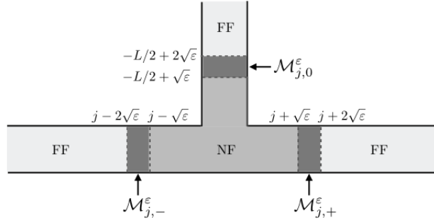
Figure 7: the matching area \mathcal{M}_{j,m}^\varepsilon = \mathcal{M}_{j,-}^\varepsilon \cup \mathcal{M}_{j,+}^\varepsilon \cup \mathcal{M}_{j,0}^\varepsilon for j \neq 0 (NF: near field, FF: far field).
