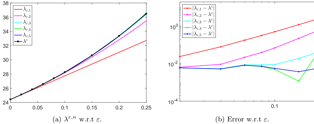
Figure 13: Results for the fourth eigenvalue.
