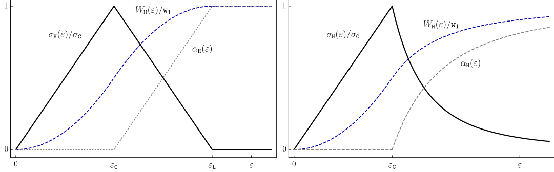
Figure 1: Homogeneous responses for the (LS), left, and (NS), right, models, for which \varepsilon_L = k\varepsilon_C and \varepsilon_L = \infty , respectively.
