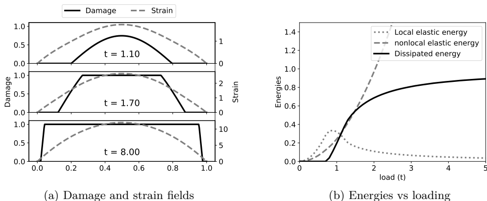
Figure 11: Strain-Gradient model LS-G1: numerical results for the traction test. The simulation is without imperfection for \eta/L = 0.2 and n = 300 elements.
