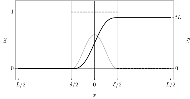
Figure 9: Minimising sequence (74) for the SG0 model with \mathbf{E}(1) = \mathbf{G}(1) = 0 . Black solid line: displacement u_\delta ; dashed line: damage \alpha_\delta ; gray solid line: strain \varepsilon_\delta .
