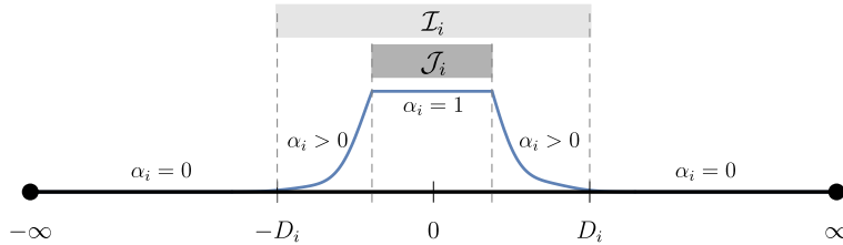
Figure 5: Sketch of the damage field in the considered non-homogenous solution.
