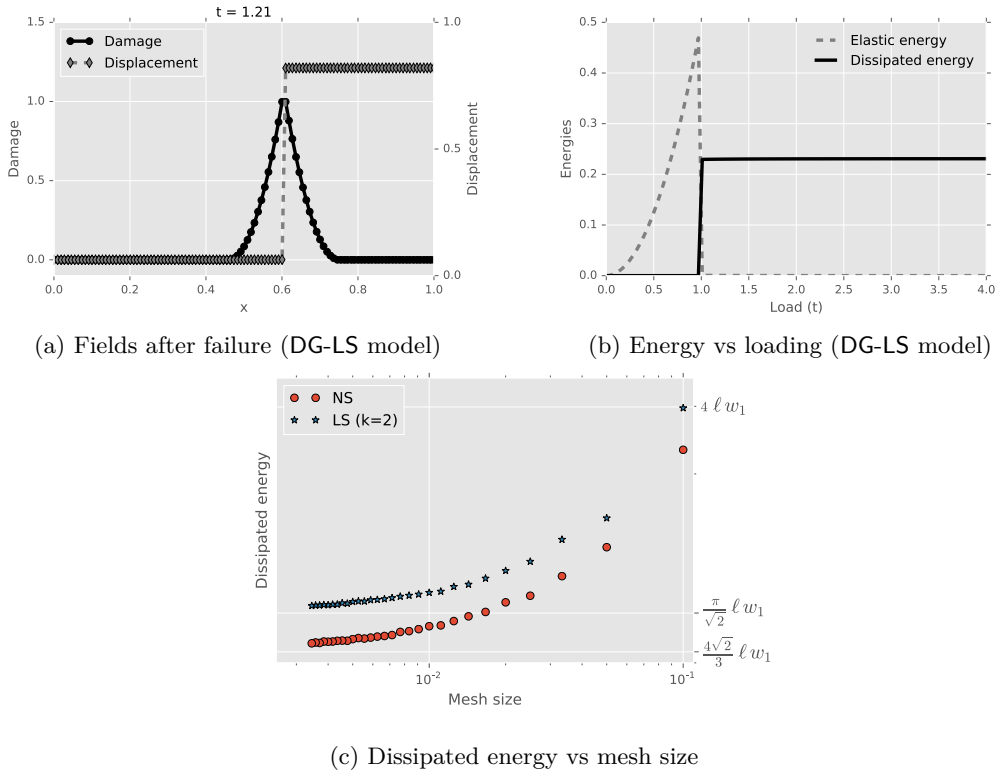
Figure 3: Damage-Gradient model: numerical results for the traction test for the (LS) and (NS) models in (24). The results are for \ell = 0.1L and a small imperfection on the Young modulus in x = 0.6L . The width of the localisation zone and the dissipated energies converge to well-defined finite values, see (37), when decreasing the mesh size. The dissipated energies after failure do not depend on the loading. Hence it is possible to associate a well-definite constant dissipated energy to a crack and the model is energetic equivalent with the Griffith fracture model.
