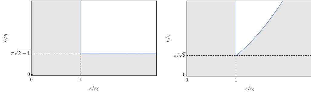
Figure 4: Conditions for the local uniqueness of the homogenous response as a function of the loading ( \varepsilon/\varepsilon_c ) and the normalized bar length ( L/\eta ). Light gray indicates regions where the homogeneous response is locally unique, hence stable. Left: (LS) model; right: (NS) model.
