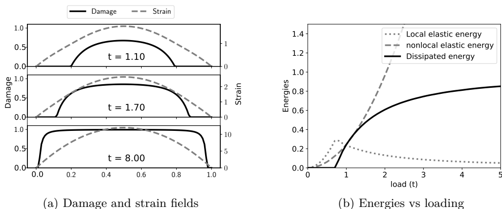
Figure 10: Strain-Gradient model NS-G1: numerical results for the traction test. The simulation is without imperfection for \eta/L = 0.2 and n = 100 elements.
