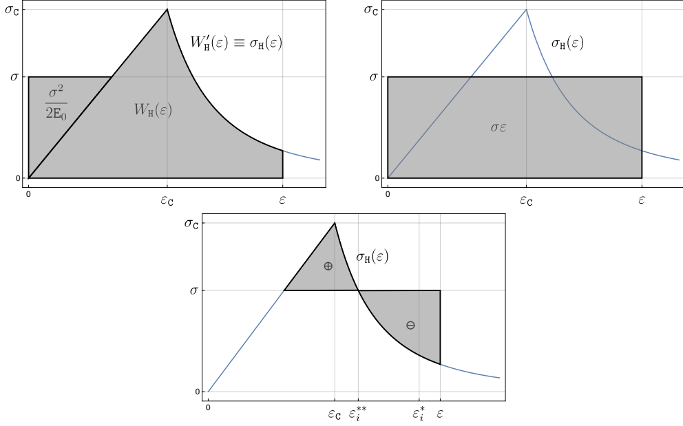
Figure B.14: Geometrical interpretation of the energetic contents defining the function F_\sigma(\varepsilon) . Upper left: (W_{\mathbb{H}}(\varepsilon) + \sigma^2/(2E_0)) . Upper right: (\sigma\varepsilon) . Bottom: the difference of the terms above, namely (E_0 F_\sigma(\varepsilon)/2) .
