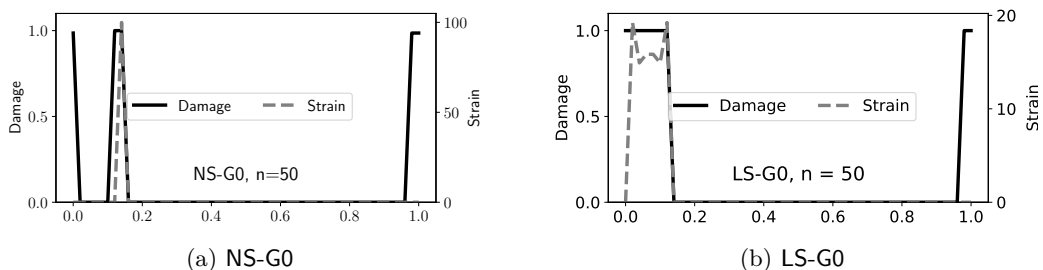
Figure 13: Strain-Gradient models SG0: the results of the numerical simulations show uncontrolled localization of the damage and strain fields and are extremely sensitive to the mesh, imperfections and solver parameters. The figures show a snapshot of the damage and strain field at t = 2.0 for \eta/L = 0.2 and n = 50 elements.
