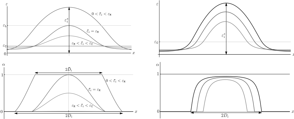
Figure 8: Evolution of the strain and damage fields for the LS model with k = 2 (Left) and for the NS model (Right) when \bar{\varepsilon}_i is decreasing from \varepsilon_c to 0.
