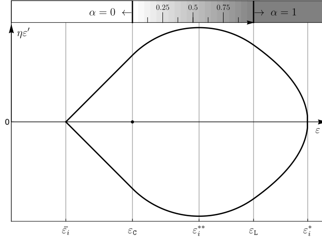
Figure 7: Plot of the localised solution curve \eta\varepsilon'_i = \pm\sqrt{F_i(\varepsilon_i)} in the (\varepsilon, \eta\varepsilon') plane when \varepsilon_i^* > \varepsilon_L . The color bar at the top of the plot gives the value of the damage field \alpha_i calculated as a function of \varepsilon_i using (14). The qualitative properties of this curve are given in Proposition 5.1.
