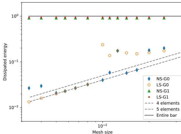
Figure 12: Strain-Gradient models: dissipated energies vs. mesh size at the end of the loading process. Markers are data from numerical simulations. The dashed and continuous lines serve as reference giving the dissipated energies corresponding to the full damage of few elements or of the whole bar.
