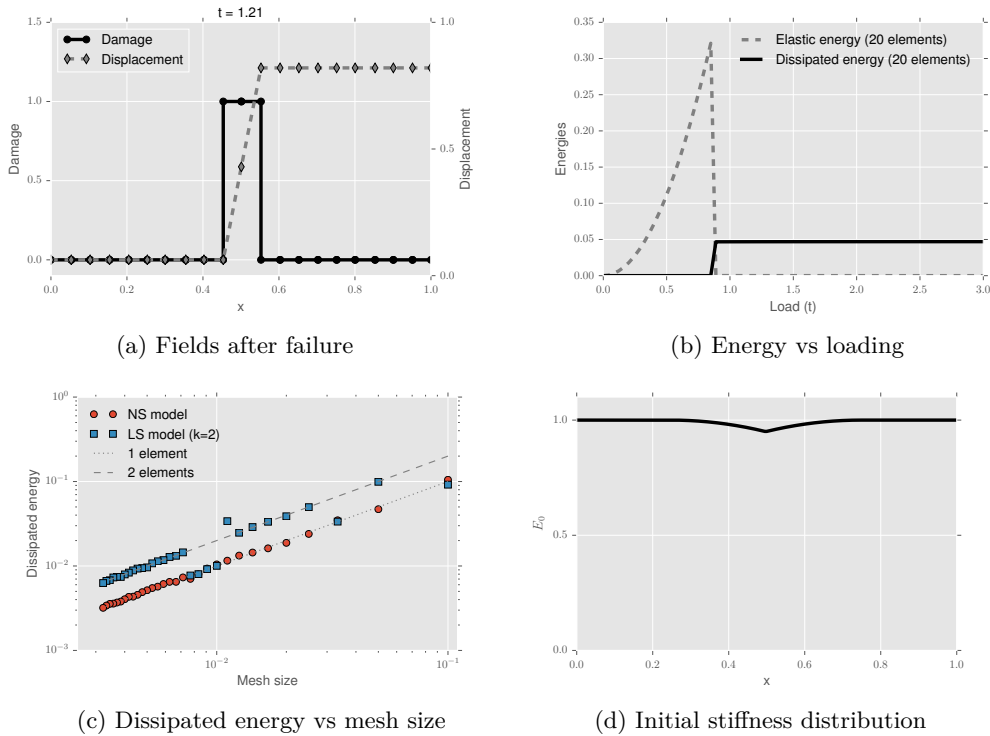
Figure 2: Numerical results for the non-homogenous traction test with the local model characterized by \mathbf{E}(\alpha) = (1 - \alpha)^2 \mathbf{E}_0 and \mathbf{w}(\alpha) = \mathbf{w}_1 \alpha . Figure 2a shows the damage and displacement fields after failure, emphasising the discretisation (markers correspond to nodes in the finite element mesh). Figure 2b reports the evolution of the energy with the loading t . Before failure ( t \simeq 1.0 ), the elastic energy is quadratic in t (elastic response) and the dissipated energy is zero. After failure, the elastic energy vanishes and the dissipated energy is strongly dependent on the mesh size. The damage localizes in a zone of a one or two elements and the dissipated energy scales linearly with the mesh size, as shown in Figure 2c for both the (LS) and (NS) models in (24). Here the dashed lines are the energy values for damage localized in one ( \mathbf{w}_1 h ) or two elements ( 2\mathbf{w}_1 h ). Figure 2d illustrates the initial stiffness used in the simulations: \mathbf{E}_0(x) = \{1 \text{ for } |x| \geq d/2; 1 - 0.05(2x/d)^2 \text{ for } |x| < d/2\} .
