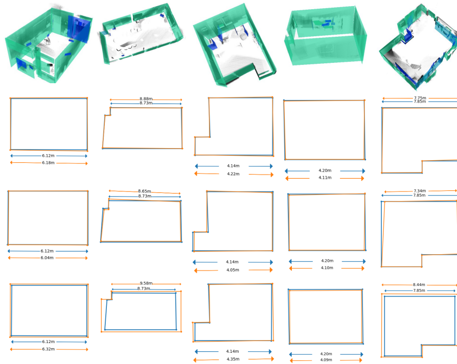
Fig. 6: First row: the point clouds and the labeled planar patches (blue: clutter, green: walls) of the scanned rooms: Lab1 MW , Lab2, House1 MW , House2 MW and House3 MW (from left to right). Second row: comparison of our approach in orange with the ground truth in blue. Third and fourth row : comparison of the room layout obtained with FloorPlanEx and Magic Plan in orange and the ground truth in blue.
