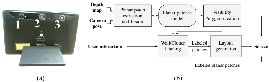
Fig. 1: (a) Tango Tablet Development Kit image sensors: RGB-IR camera (1), Fisheye camera (2), IR pattern emitter (3). (b) Our pipeline.
