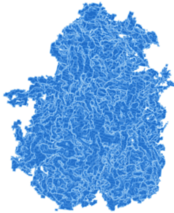
Figure 15: 3D view of the tomographic reconstruction of a small portion of mesoporous alumina. The image has a 0.87 nm voxel size, and the image field of view is 328 nm \times 290 nm \times 257 nm.
