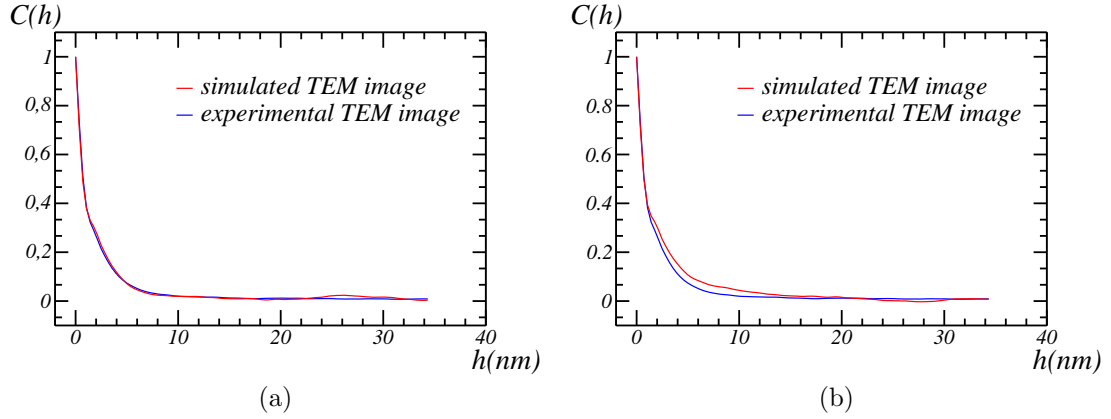
Figure 24: Experimental and simulated correlation functions of (a) the two-scale model and (b) the three-scale model of platelets for mesoporous alumina. The parameters of the microstructures are shown in Table 1.
