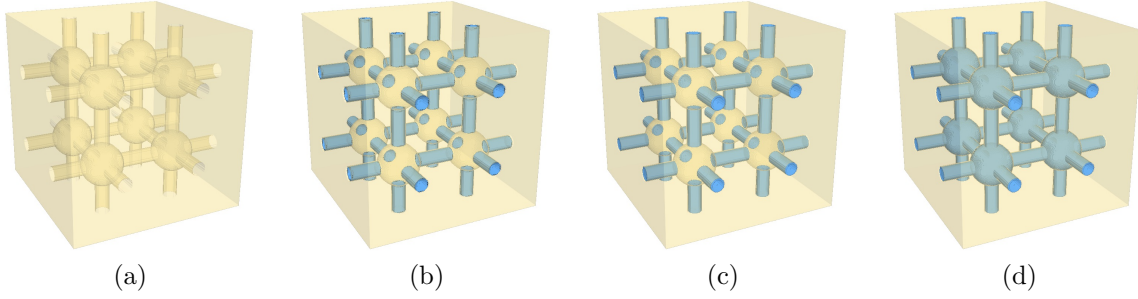
Figure 6: Condensation in a regular cylinder-sphere grid pore.
