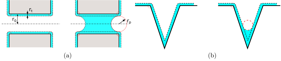
Figure 3: 2D sections of cylindrical (a) and conical (b) pores with multilayer adsorption (left images) and capillary condensation (right images). Solid phase is in grey. Liquid phase is in blue. Red dotted lines are the structuring elements.
