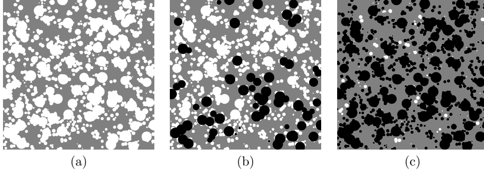
Figure A.29: Desorption process of the two-scale model with spherical pores. Maps (a), (b) and (c) correspond to r_p = 37, 36 and 12 voxels respectively (see Fig. A.28).
