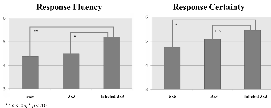
Figure 3: Univariate analysis results
