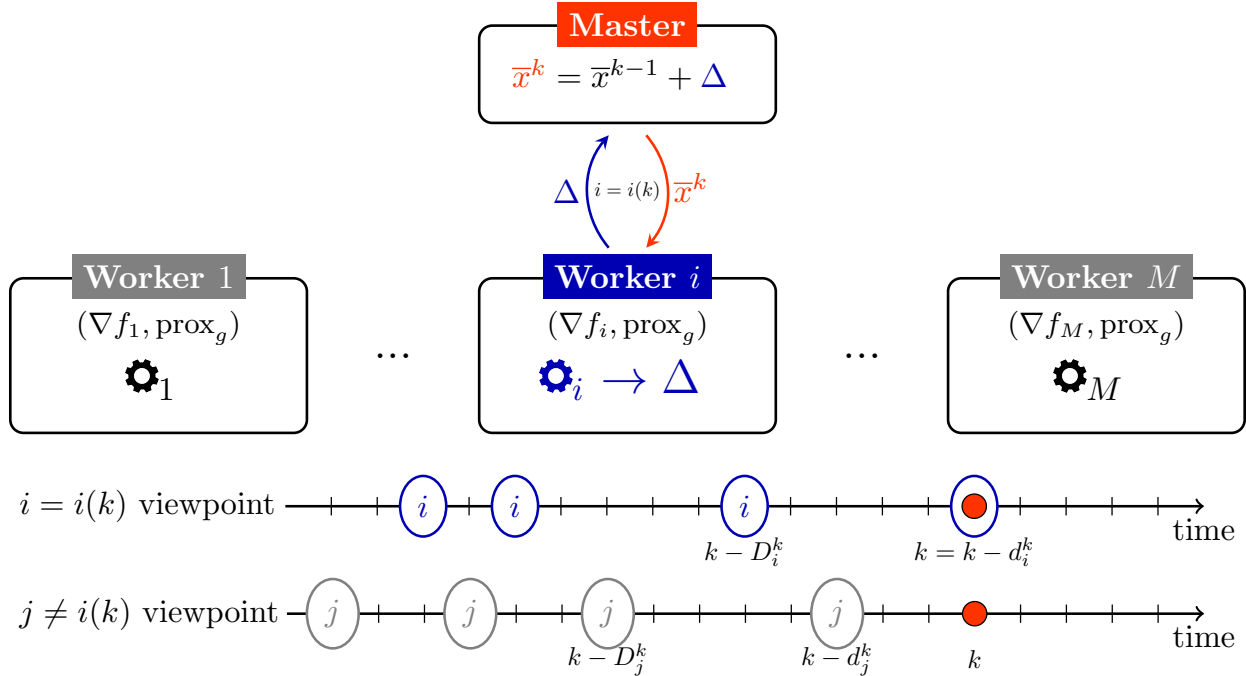
Figure 1: Asynchronous distributed setting and delays notation.
