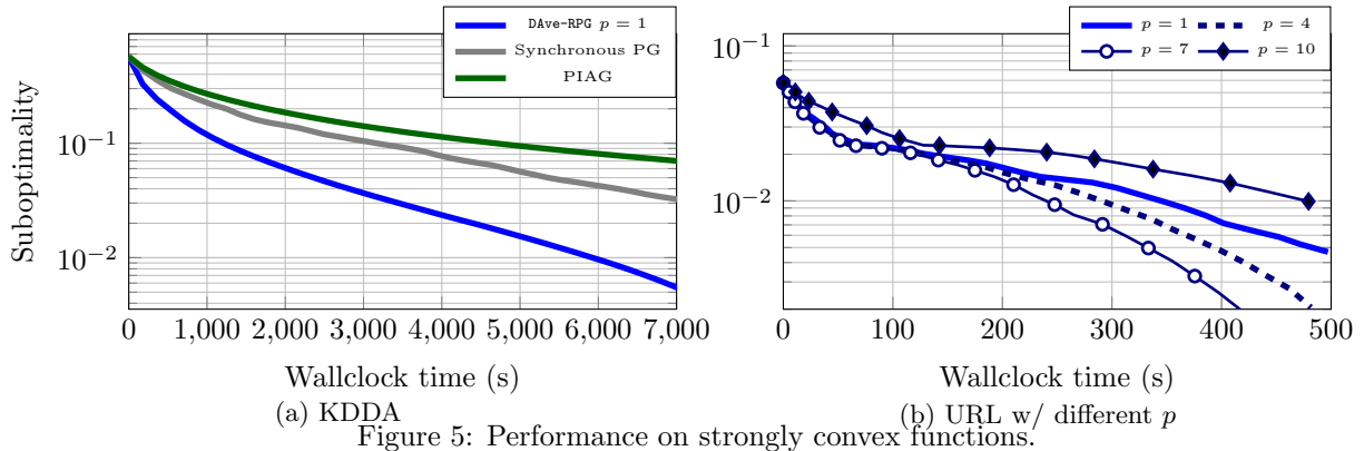
Figure 5: Performance on strongly convex functions.
