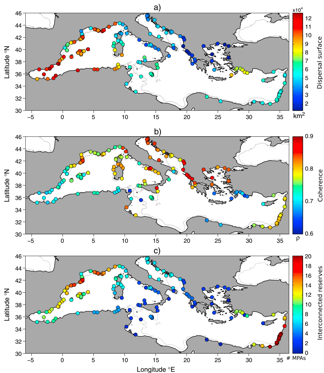
Figure 3. Spatial variability of MPAs connectivity derived from three complementary metrics averaged across all winter/summer experiments over 2002–2011 using \tau \approx \text{PLD} = 30 days. (a) Mean area (in \text{km}^2 ) and (b) mean \rho of the province sheltering the reserve of interest. (c) Mean number of interconnected MPAs (i.e. number of reserves situated within the same hydrodynamical province). Light grey contours represent the 200 m isobath. Results using a PLD of 45 and 60 days are qualitatively similar with a slight increase of the mean area and the number of interconnected reserves. Note that noncontiguous areas belonging administratively to a given reserve were treated here as a single MPA.
