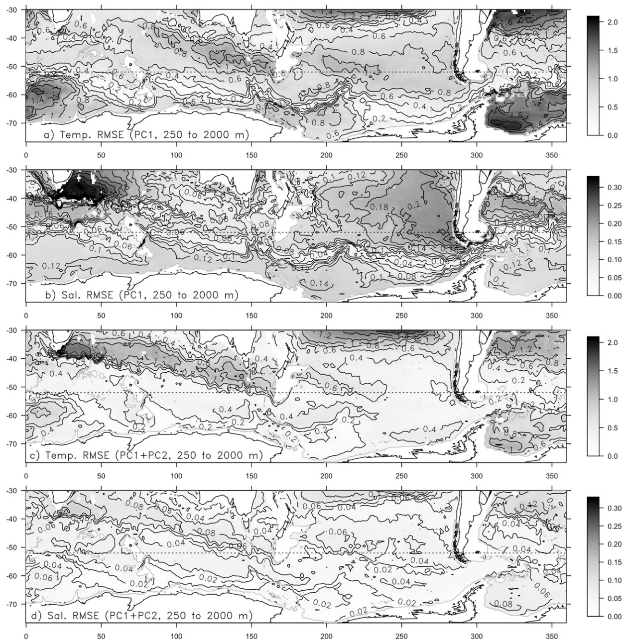
FIG. 10. Vertical RMSE of the profiles reconstructed with (a),(b) PC1 and (c),(d) PC1 + PC2 for temperature ( ^{\circ}\text{C} ) and salinity (psu) from 250 to 2000 m. The dotted line is at 52^{\circ}\text{S} , illustrating the regional separation used in Fig. 9.
