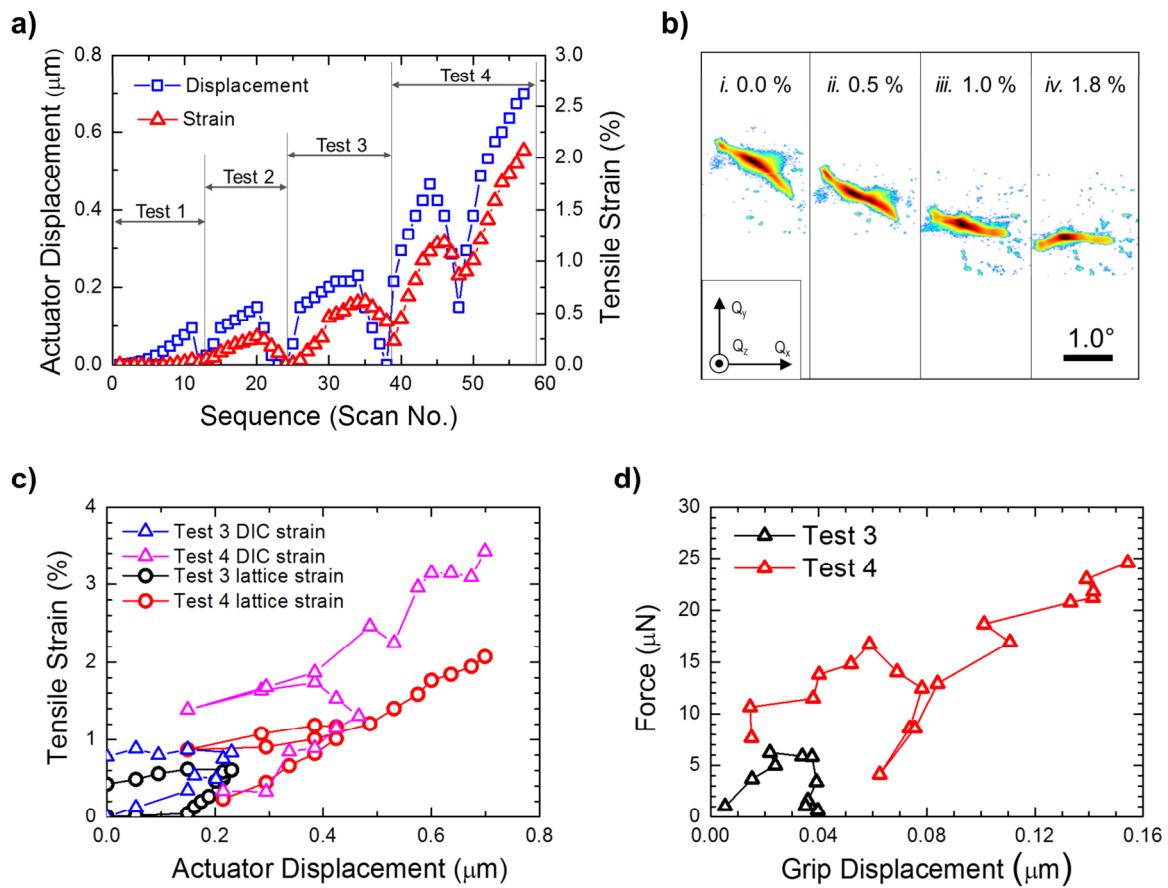
Figure 2. a) [0\ \bar{1}\ 1] tensile strain response overlaid with the applied actuator displacement during the tests. b) Evolution of the shape from Q_z sum of 311 Bragg peak at 0%, 0.5%, 1% and 1.8% tensile strain. c) Comparison of strain measured with DIC and the lattice strain from Bragg peak analysis d) Load-displacement curve
