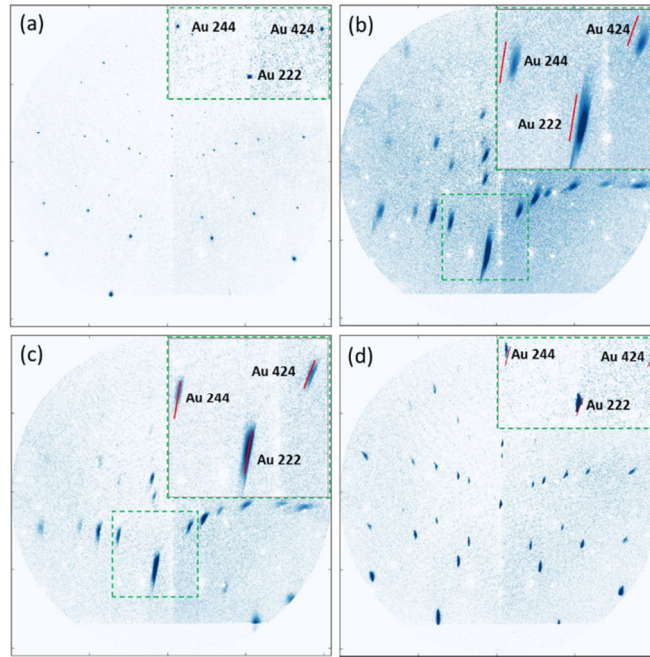
Fig. 3: Laue microdiffraction patterns taken (a) at the reference position ( Y=4.4\ \mu\text{m} ), (b) at the left-hand side and (c) at the right-hand side of the largest bending angle ( Y=16.4, 17.4\ \mu\text{m} ), and (d) at the right-hand side of the loading position ( Y=19.9\ \mu\text{m} ). The positions where these diffraction patterns were recorded are indicated by arrows in Figs. 2(b) and (d).
